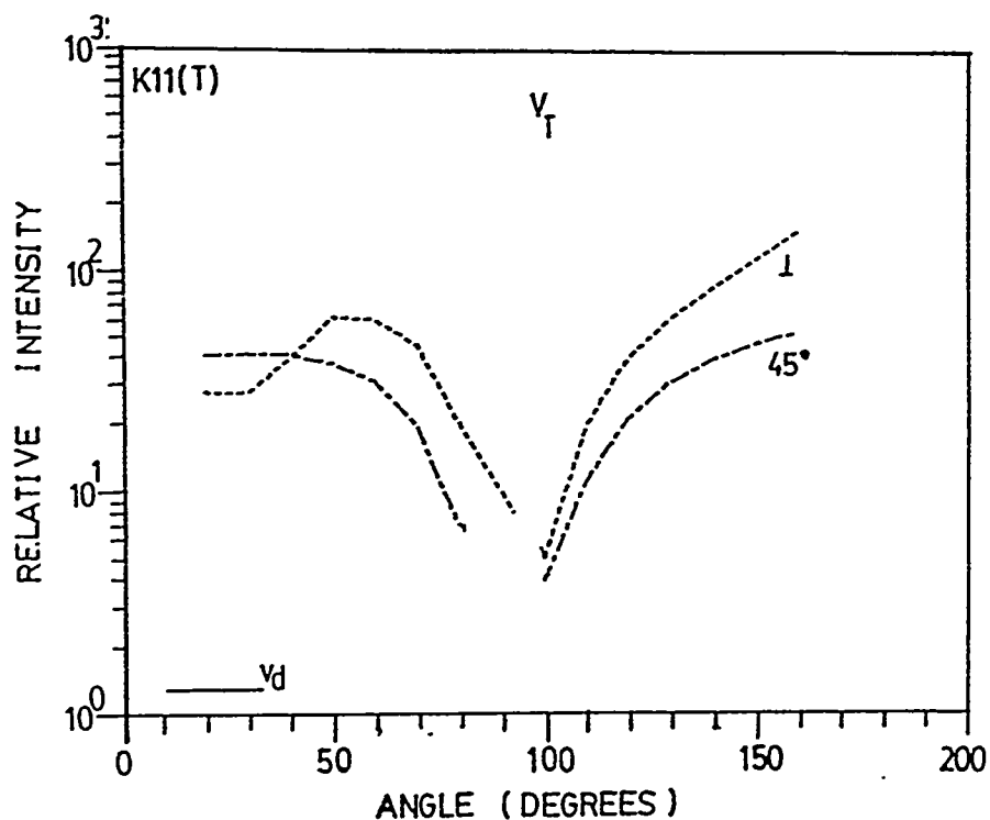
Figure 5.20. Angular distribution of fluorescent scattering from sample K11 treated Oxazine, for vertically polarized incident light. The sample was aligned at 45^\circ and 90^\circ to the incident beam. The cone bases are up stream.
