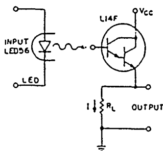
5. TEST CIRCUIT
