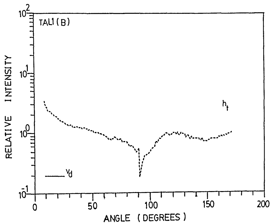
Figure 5.8. Angular distribution of fluorescent scattering from sample TAL1 treated Oxazine, for horizontally polarized incident light, at base-on incidence.
