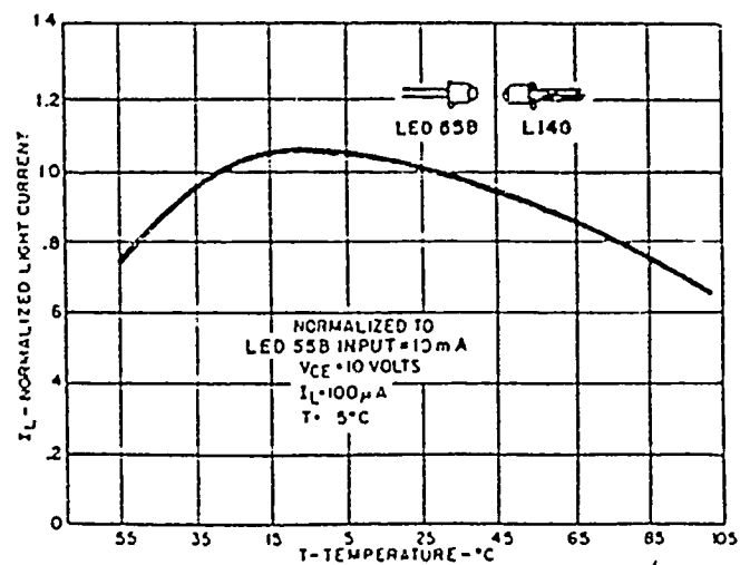
Normalized Light Current vs Temperature Both Emitter (LED55B) and Detector (L14G) at Same Temperature
