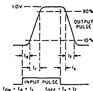
6. WAVE FORMS
