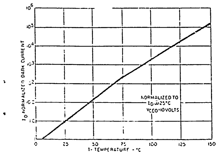
Dark Current vs Temperature
