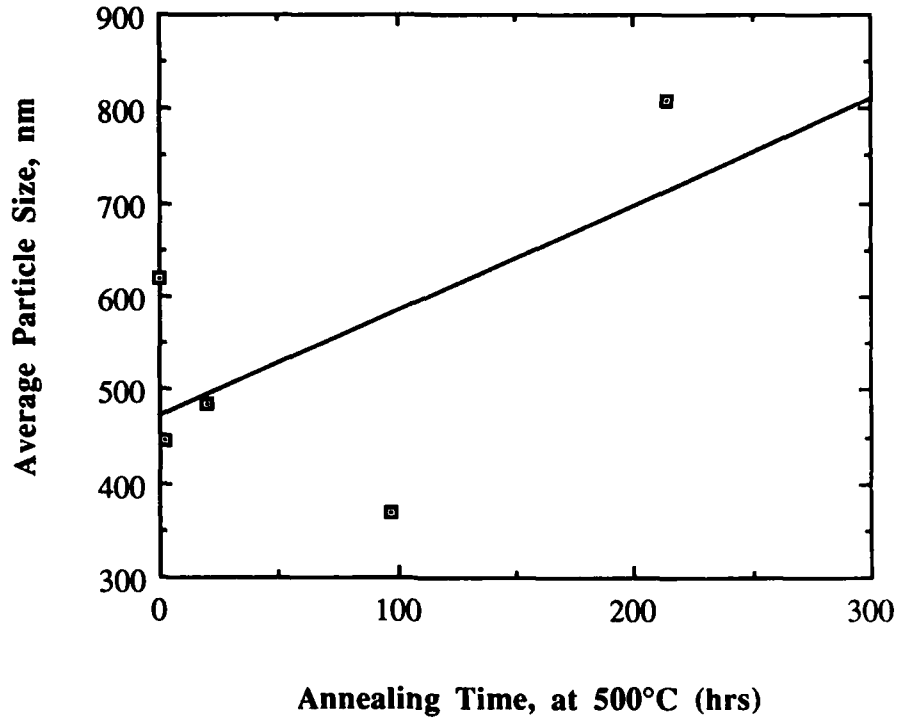
Figure 5. Variations in the average size of the Al_3Ti precipitates with thermal exposure at 500^\circ C in the unreinforced hot extruded material.
