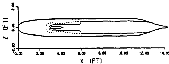
Fig. 11. Crossflow separation patterns on a submarine hull/sail configuration at \alpha = 15^\circ : (a) side view, (b) top view. Solid line denotes the terminal line.
