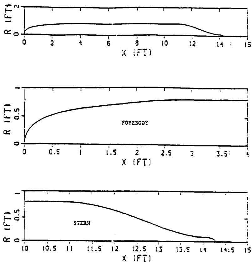
Fig. 4. Hull profile.
