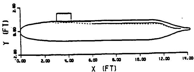
Fig. 11. Crossflow separation patterns on a submarine hull/sail configuration at \alpha = 15^\circ : (a) side view, (b) top view. Solid line denotes the terminal line.
