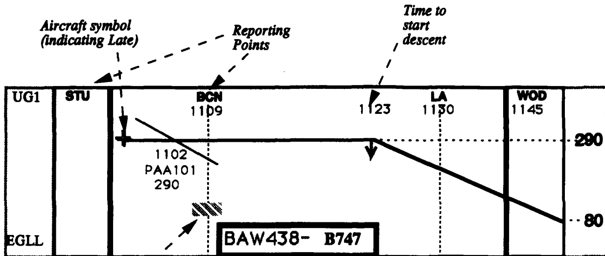
PROFILE DATA STRIP - EASTBOUND
