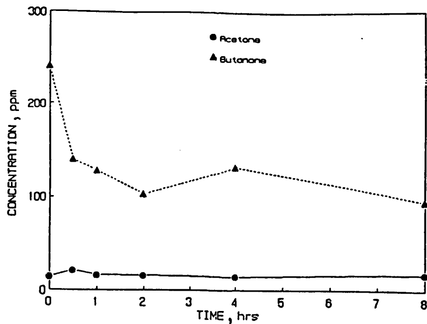
Figure 39. Acetone and butanone AC equilibrium data (concentrated plot)
