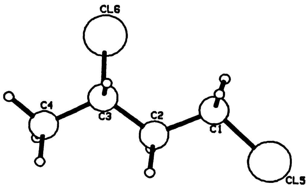
1, 3 - CHLORO BUTANE (Dimer)
