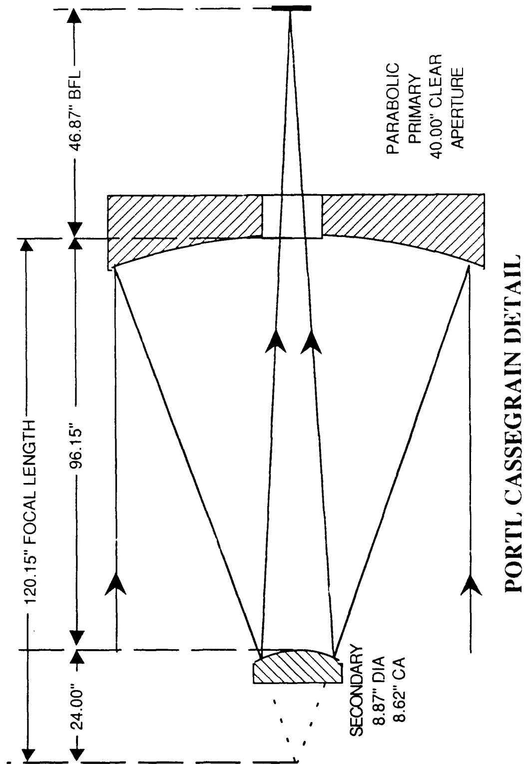
Figure 2. PORTL Optical Prescription
