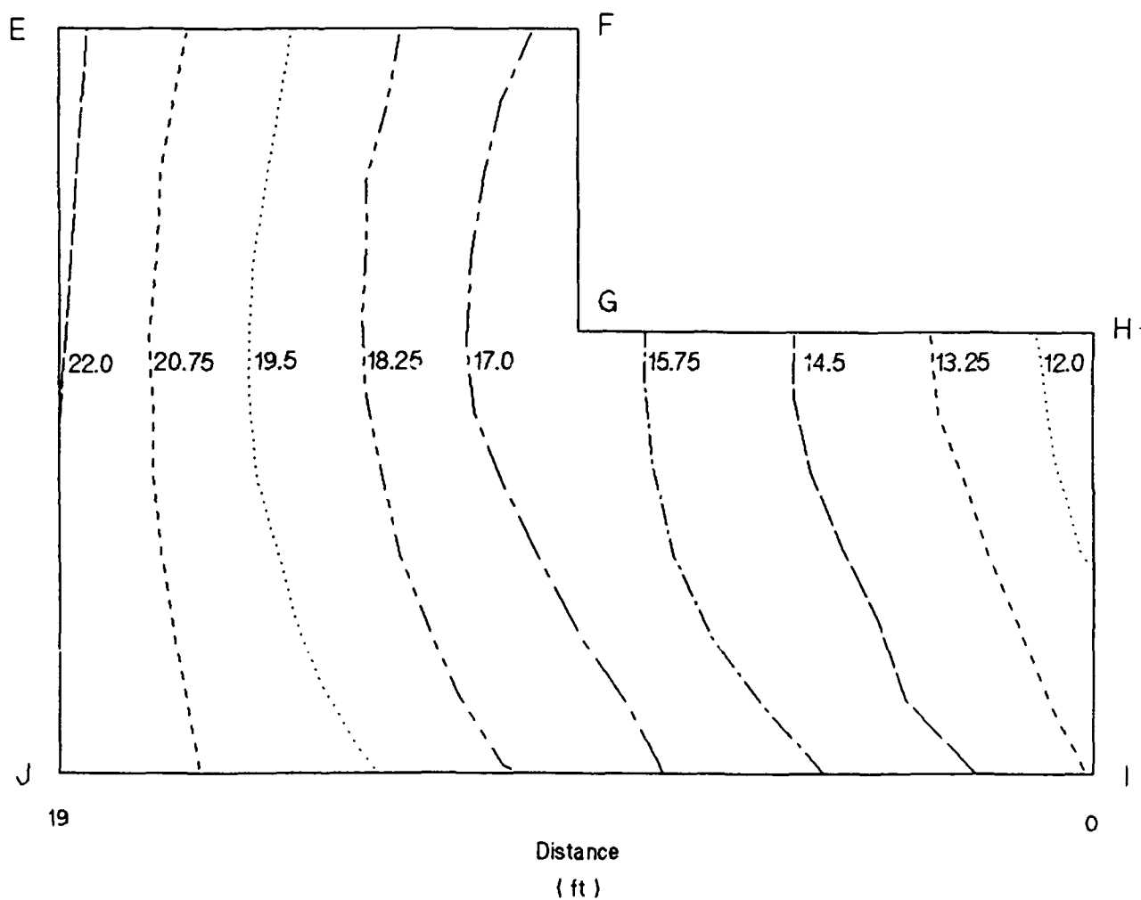
Figure 34. Temperature ( ^{\circ}\text{F} ) amplitudes in land wall. See Figure 30 for orientation of this section
