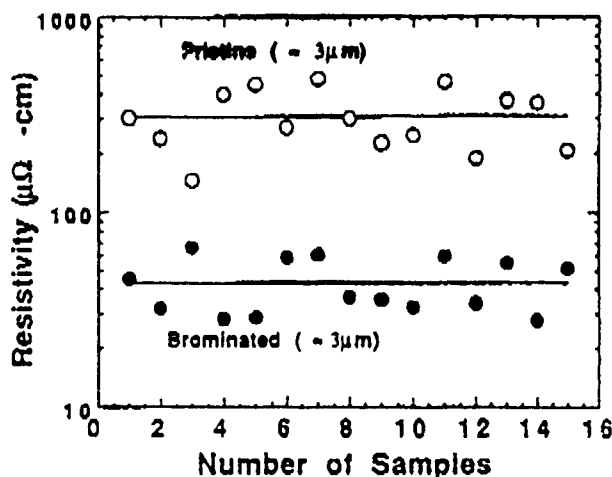
Figure 3 Results of the resistivity measurements on a number of smaller (2.7 μm) fibers.
