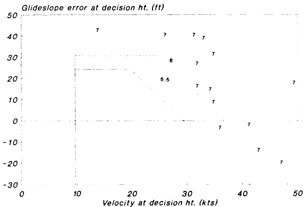
FIG. 14: HANDLING QUALITIES RATINGS FOR 9° GLIDESLOPE APPROACHES WHEN \Delta \dot{e} > 7.0 ft/sec
