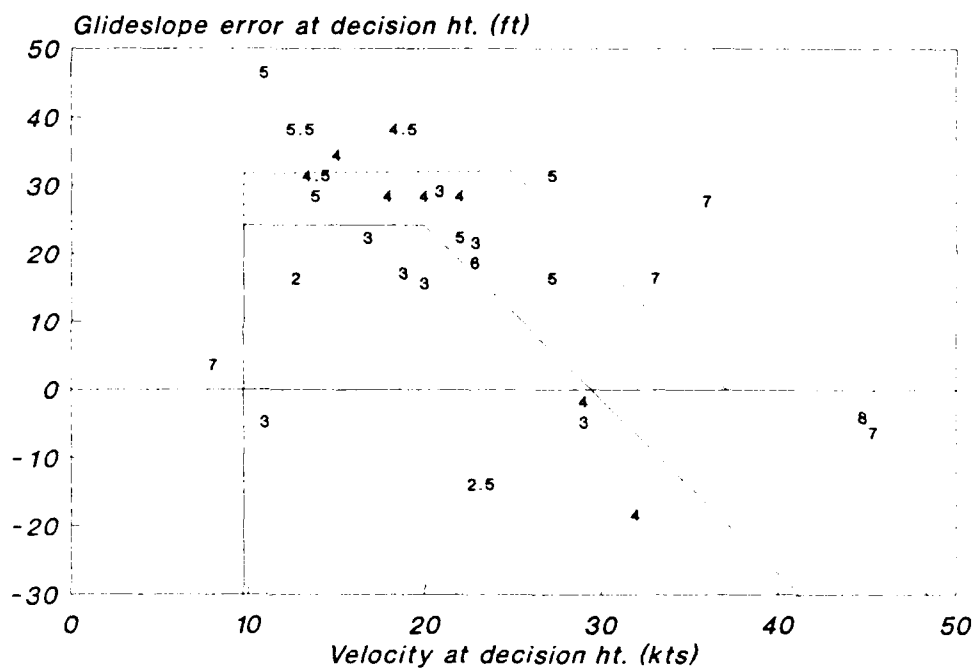
FIG. 13: HANDLING QUALITIES RATINGS FOR 9° GLIDESLOPE APPROACHES WHEN 3.5 < \Delta \dot{e} < 7.0 ft/sec
