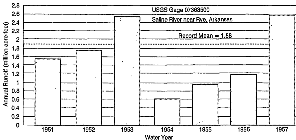
Figure 45. Comparison of PHDI, Precipitation and Runoff for 1953-56 Drought
