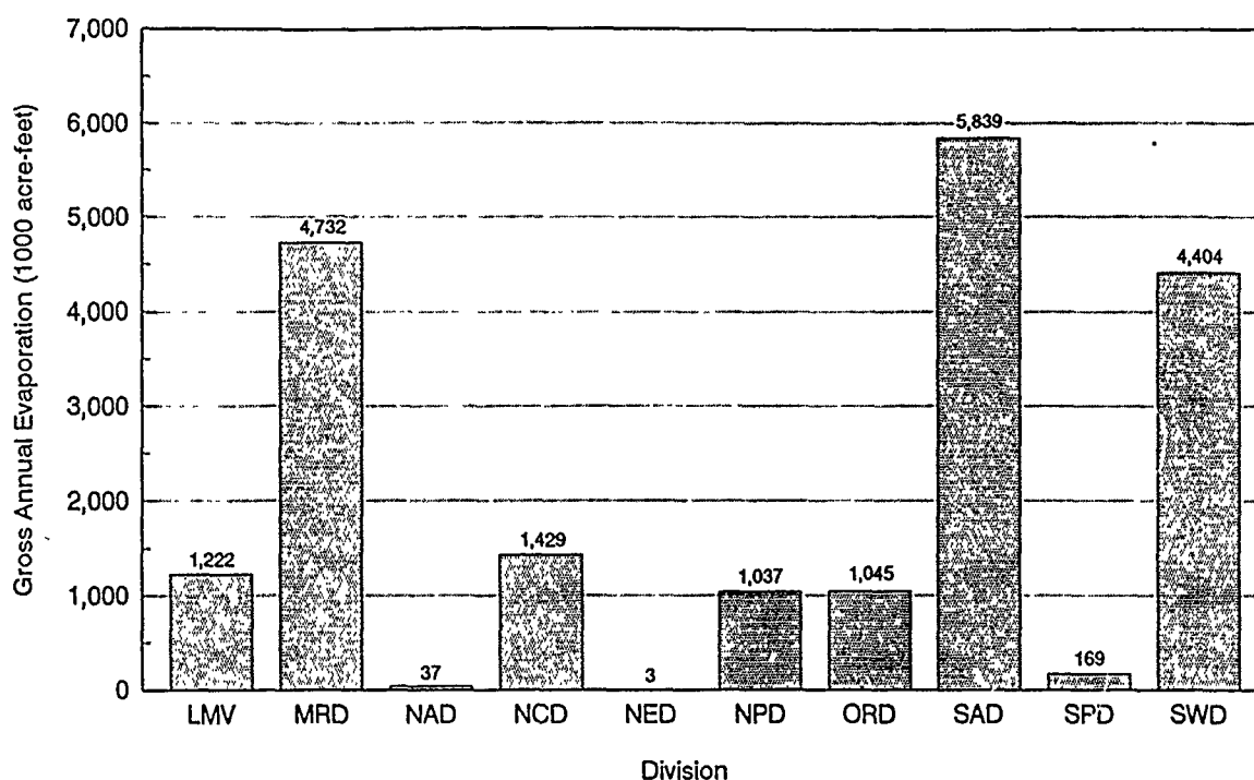
Figure 11. Gross Annual Reservoir Evaporation by Division
