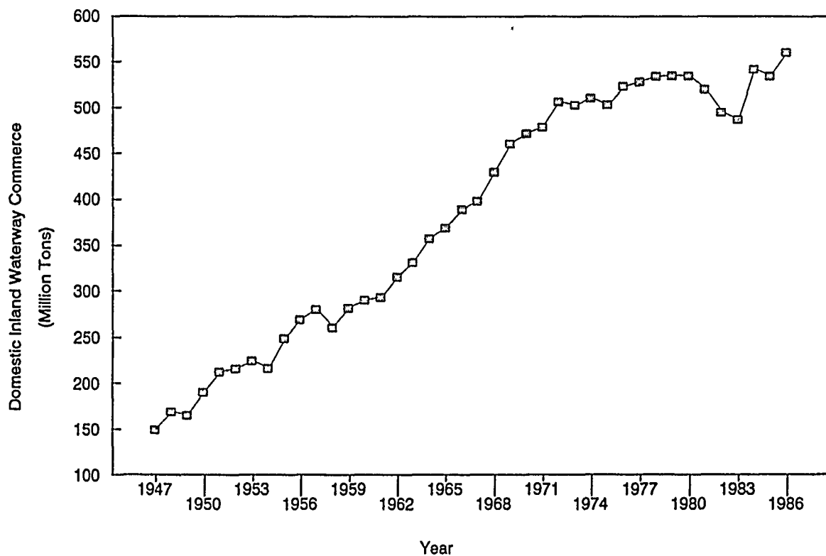
Figure 16. U.S. Inland Waterway Traffic Source: Corps of Engineers, Waterborne Commerce of the United States, Annual Report 1987
