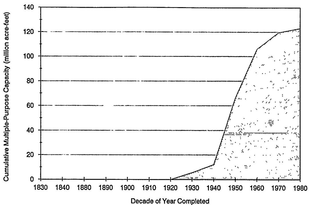
Figure 6. Growth of Reservoir Multiple-Purpose Capacity
