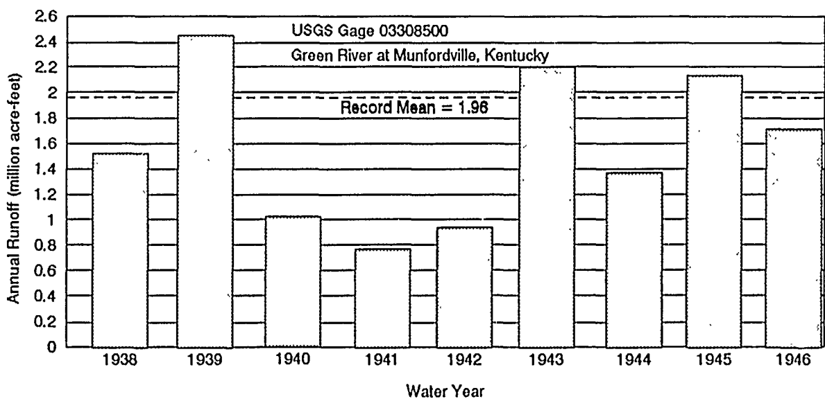
Figure 39. Comparison of PHDI, Precipitation, and Runoff for 1939-42 Drought
