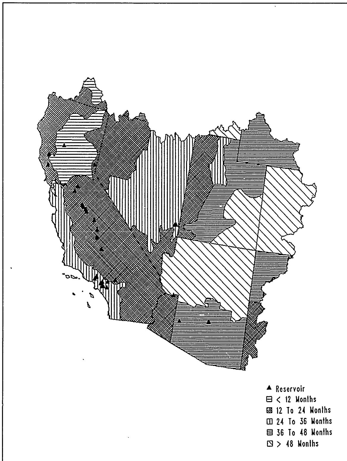
Figure 55. South Pacific Division. Climate Divisions with Severe or Extreme Drought of Different Durations (PHDI)
