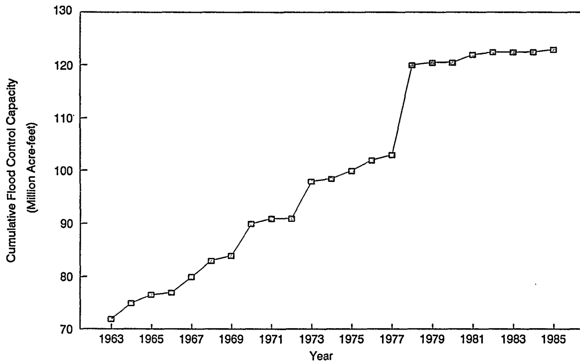
Figure 15. Cumulative Flood Control Capacity in Corps of Engineers' Reservoirs Source: U. S. Army Corps of Engineers, Annual Reports of the Chief of Engineers for Civil Works
