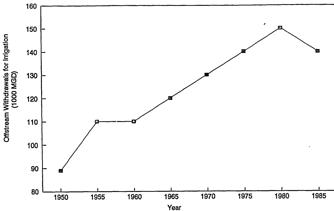
Figure 19: Irrigation Offstream Water Withdrawals
