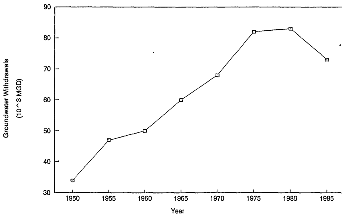
Figure 21. Groundwater Withdrawals Source: Solley et al, 1988
