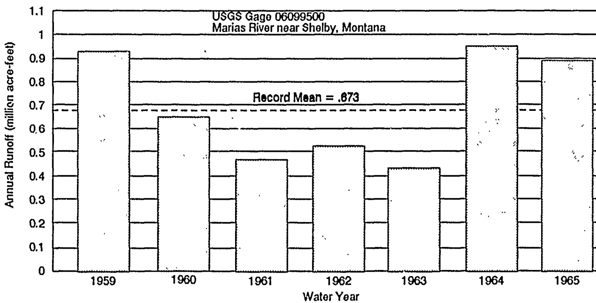
Figure 51. Comparison of PHDI, Precipitation, and Runoff for 1960-64 Drought
