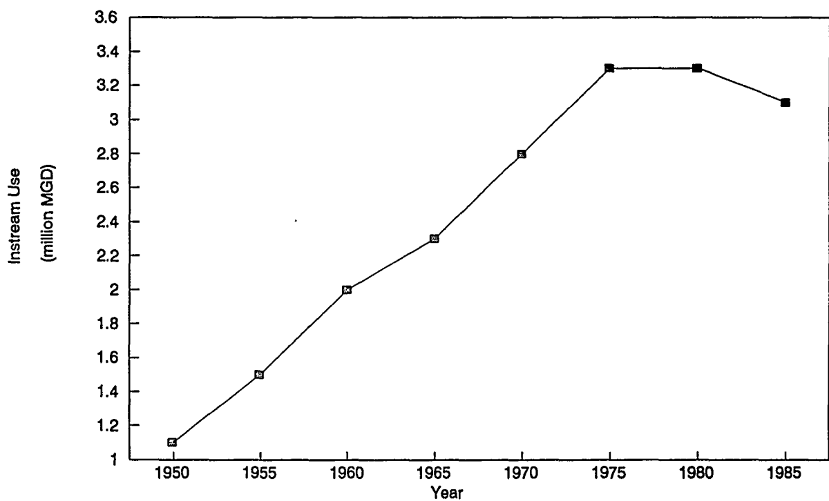
Figure 17. Hydroelectric Instream Use
