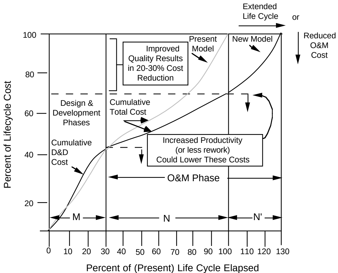
Figure 1-1: Benefits of a Mature Software Engineering Process
