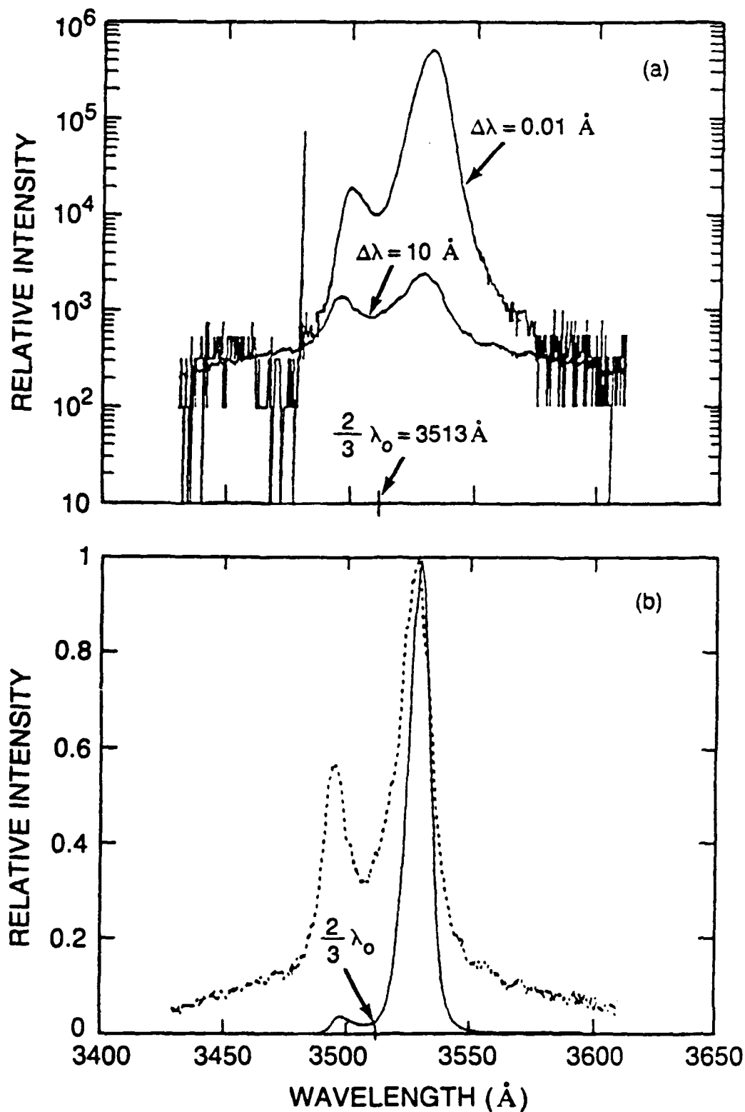
Fig. 2 — (a) Time-integrated spectra of the 3\omega_0/2 emission at the 150 degree observation angle for two shots with ISI echelons: one, at narrow bandwidth 0.01 \text{ Å} ; the other, broad bandwidth 10 \text{ Å} ; (b) The same spectra, narrow bandwidth 0.01 \text{ Å} (——) and broad bandwidth 10 \text{ Å} (-----) shown normalized to their maximum values. The wavelength corresponding to the 3\omega_0/2 frequency is indicated as 2\lambda_0/3 .
