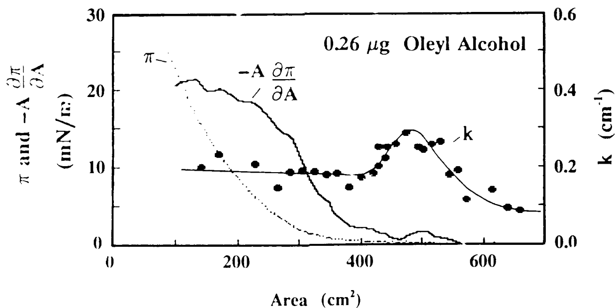
Fig. 2 - Oleyl Alcohol Monolayer: Film pressure \pi , modulus -A(\partial\pi/\partial A) , and damping coefficient k for 30 Hz capillary waves as a function of the area occupied by 0.26 \mu g of oleyl alcohol
