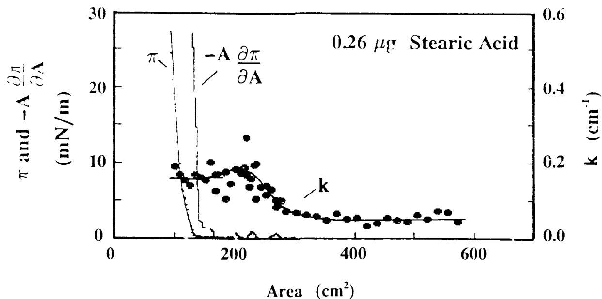
Fig. 1 - Stearic Acid Monolayer: Film pressure \pi , modulus -A(\partial\pi/\partial A) , and damping coefficient k for 30 Hz capillary waves as a function of the area occupied by 0.26 \mu g of stearic acid
