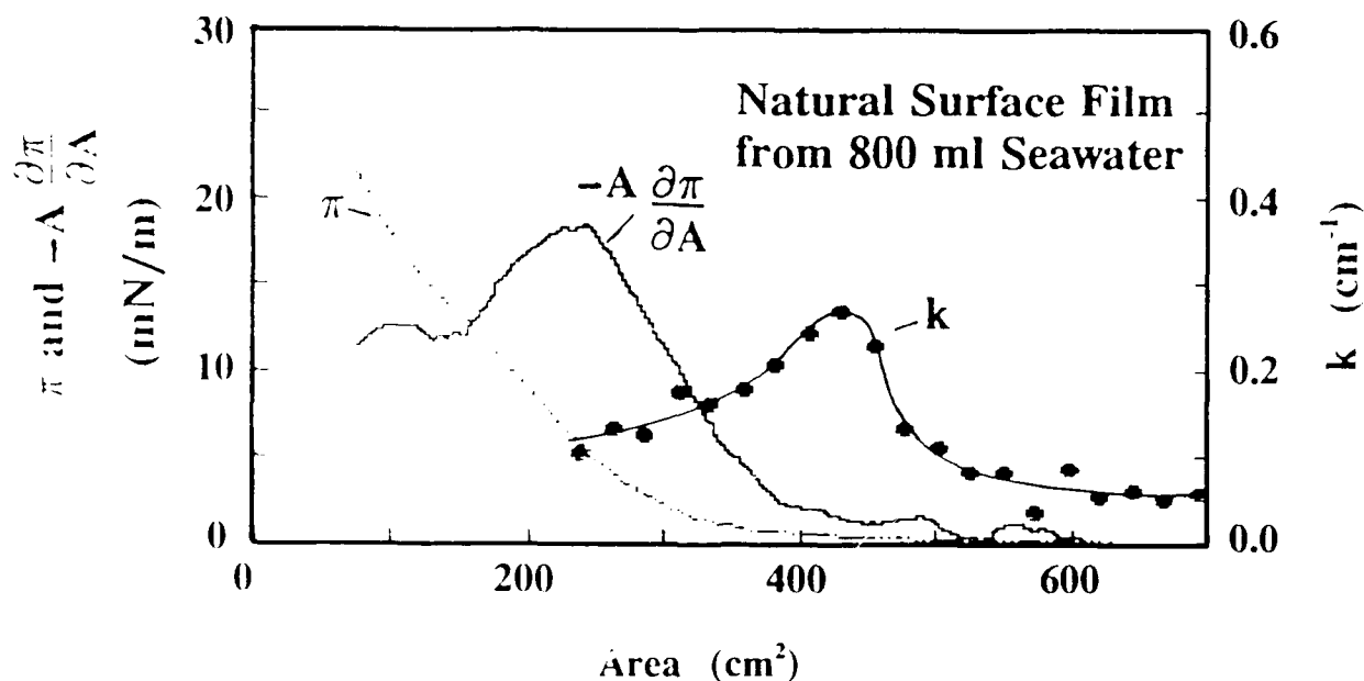
Fig. 3 - Natural Surface Film : Film pressure \pi , modulus -A(\partial\pi/\partial A) , and damping coefficient k for 30 Hz capillary waves as a function of the area occupied by the film formed on the surface of an 800 ml sample of seawater after standing overnight
