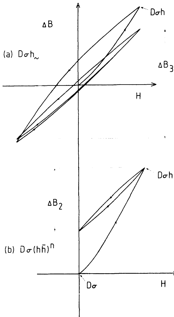
Figure 8: Schematic diagrams showing the increase in magnetization of steel subjected to the D\sigma h_{\sim} and D\sigma(h\bar{h})^n processes (up to the point D\sigma h the processes are identical).
