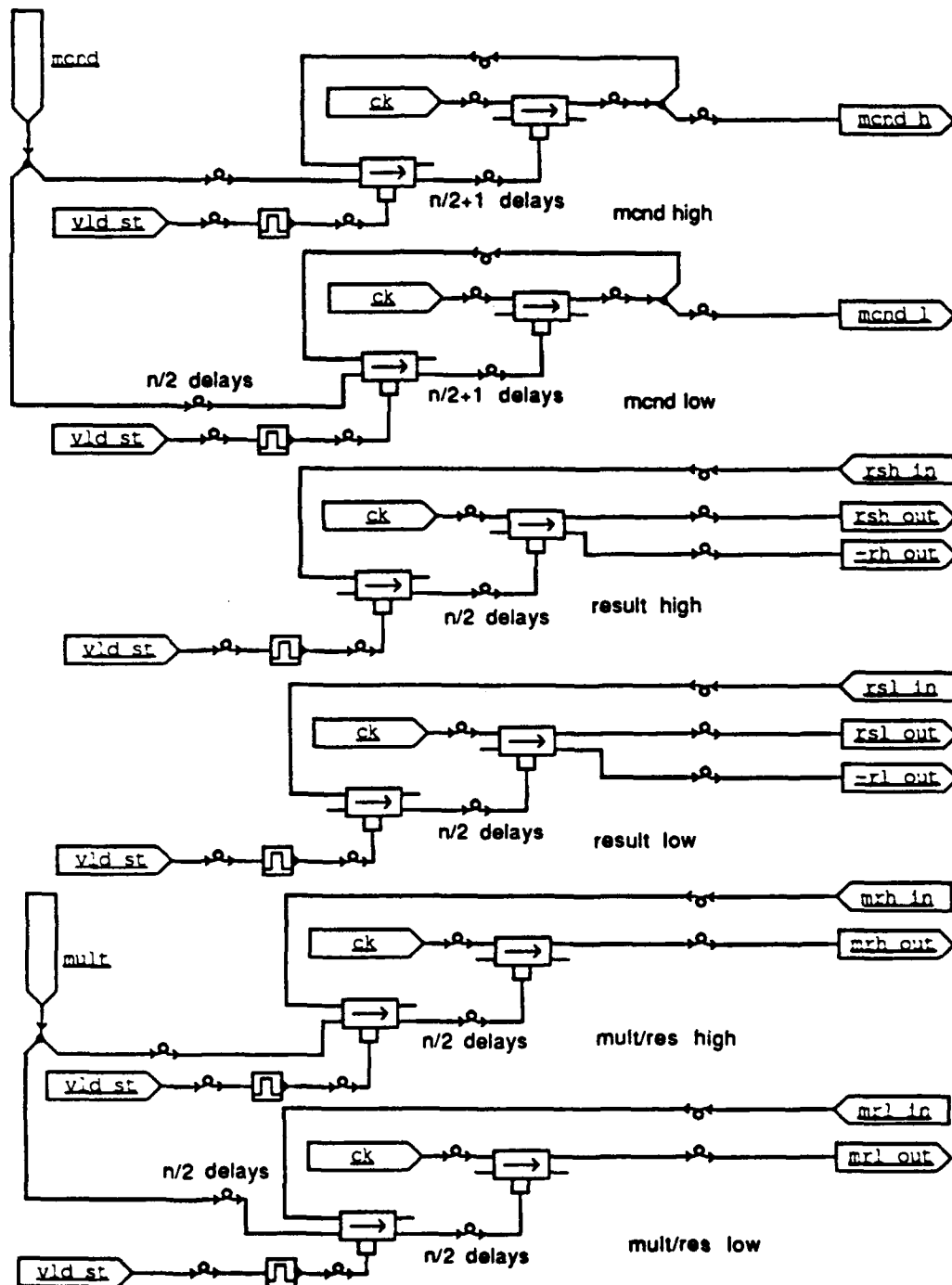
Figure B-2. Delay Lines for the High/Low Multiplier.
