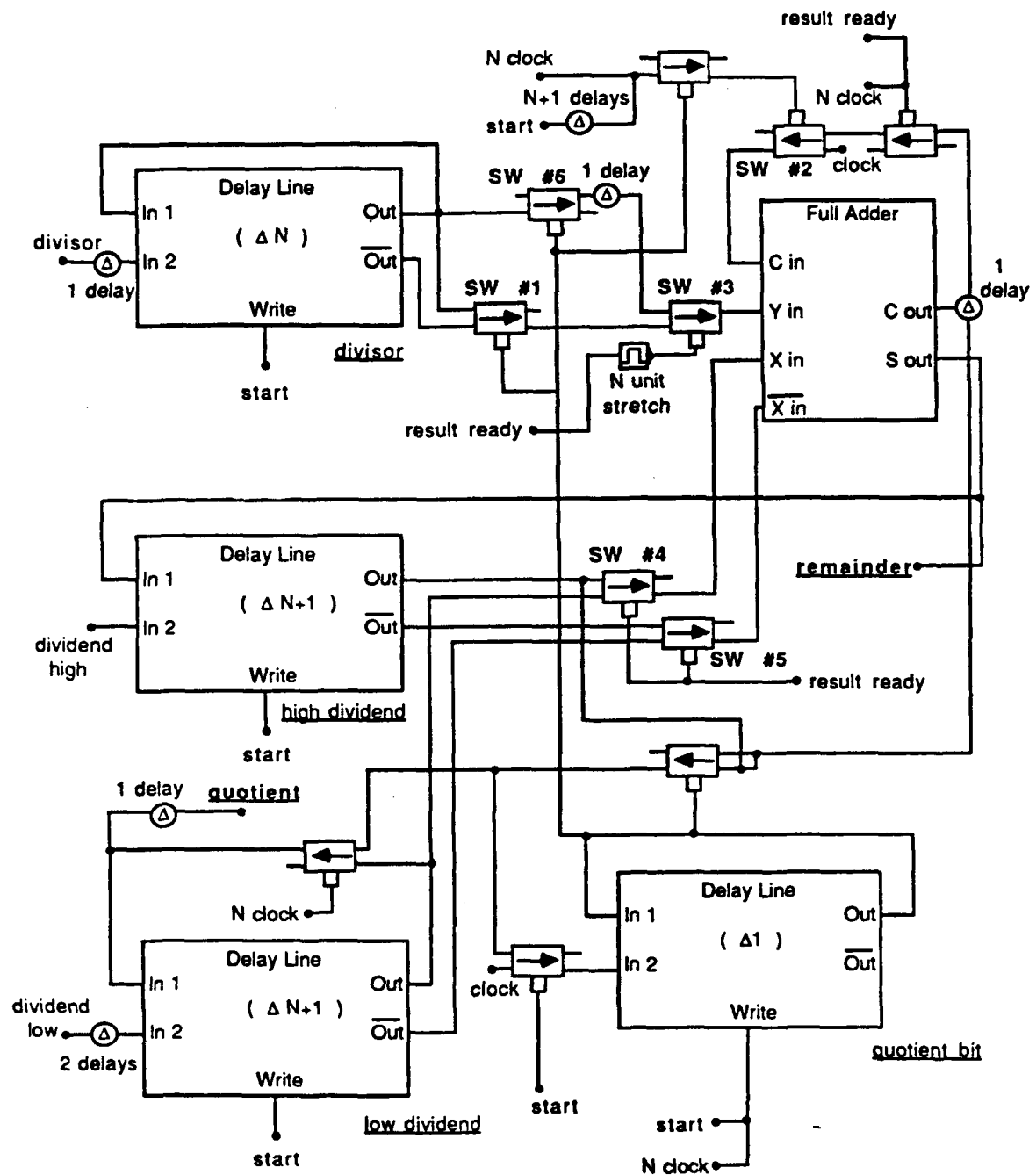
Figure 3. Non-Restoring Divider.
