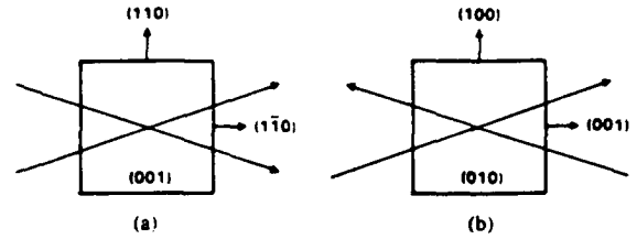
Fig. 7. (a) A configuration for codirectional cross polarization coupling in a cubic crystal of point group symmetry 43m . (b) a configuration for contradirectional cross polarization coupling in the same class of crystals.
