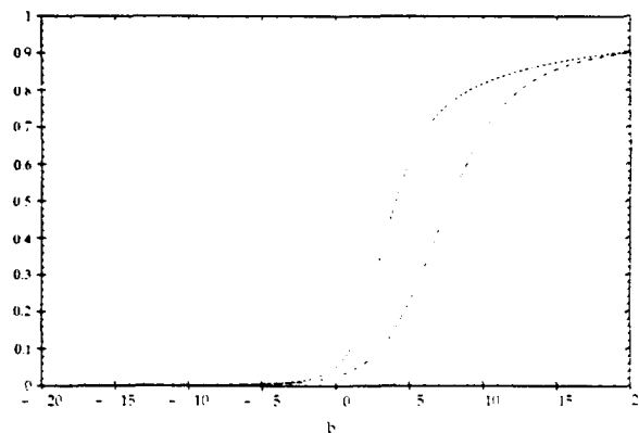
Fig. 12. Diffraction efficiency as a function of b for reflection absorption gratings ( \kappa = 0 ) with various values of \alpha L . Dotted curve, \alpha L = 2/3 ; dotted-dashed curve, \alpha L = 1 ; dashed curve, \alpha L = 2 .
