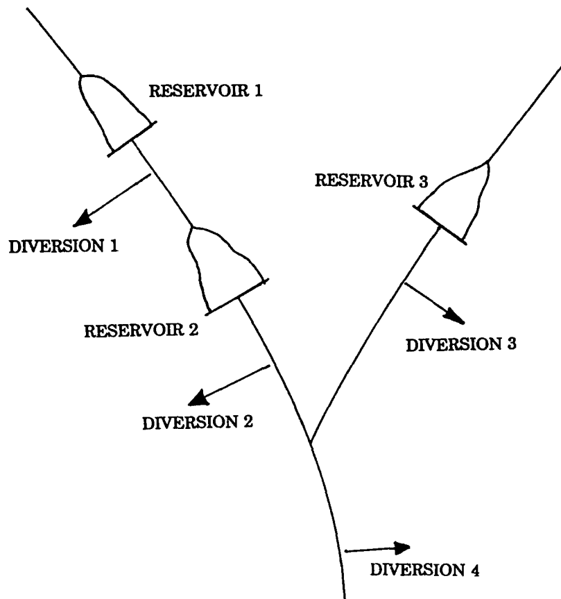
Figure 5. Multiple-Reservoir System
