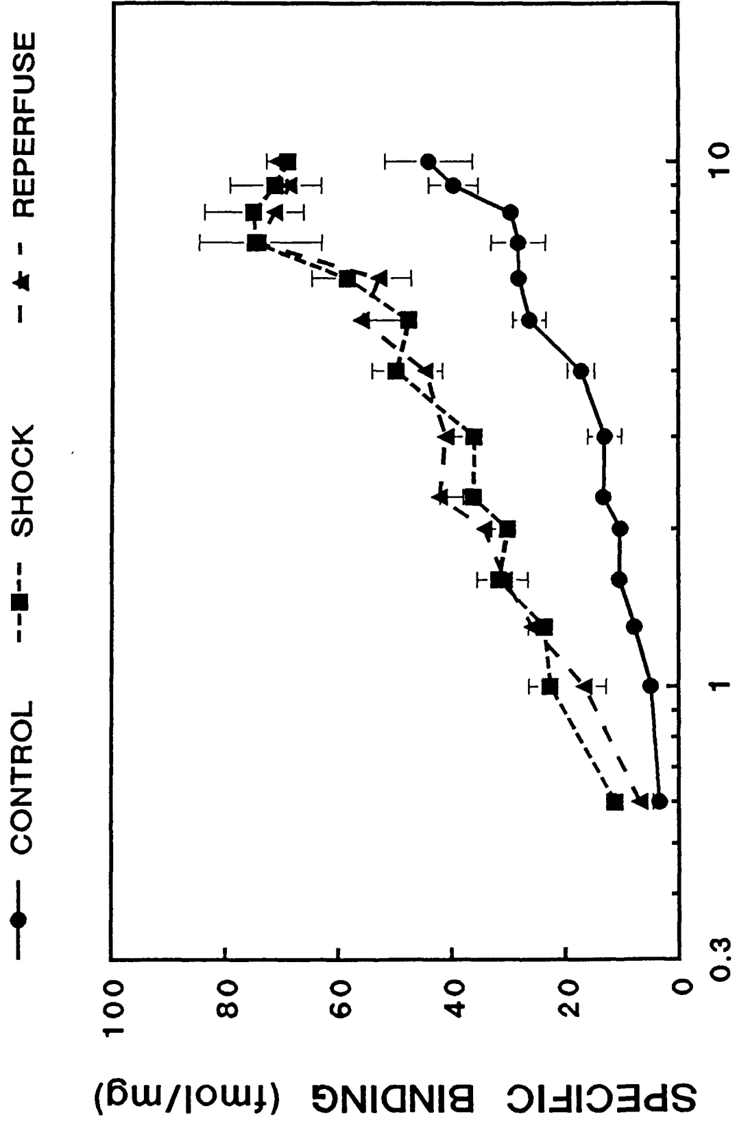
DIHYDROALPRENOLOL (nM)
