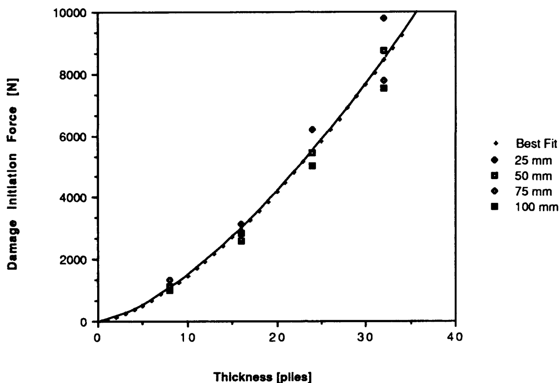
Figure 4.2. AS-4/APC-2 static data.
