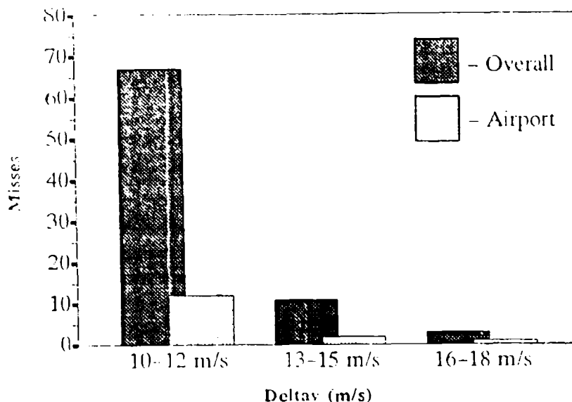
Figure 2-3. Velocity statistics for 1990 Orlando algorithm misses.
