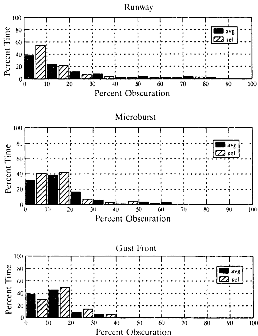
Figure 4-3. Orlando obscuration-10 heavy obscuration days.
