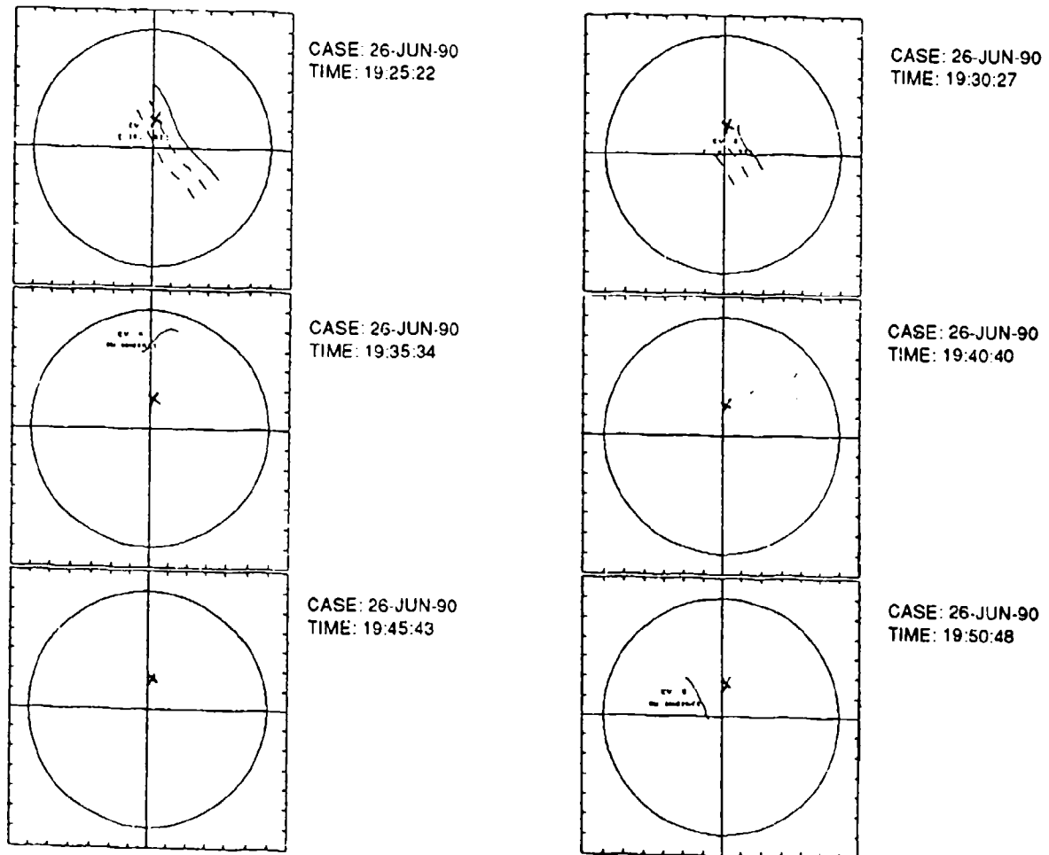
Figure 3-2. Example of the loss of a gust front detection as the gust front passes over the radar and airport. The location of the Orlando International Airport is shown by the "x." The plotting range is 30 km. The solid line indicates the current location of the gust front as determined by the algorithm. The dashed lines are the 10- and 20-minute forecasted gust front locations. The estimated wind speed (m/s) and direction (degrees) behind the gust front are shown in square brackets.
