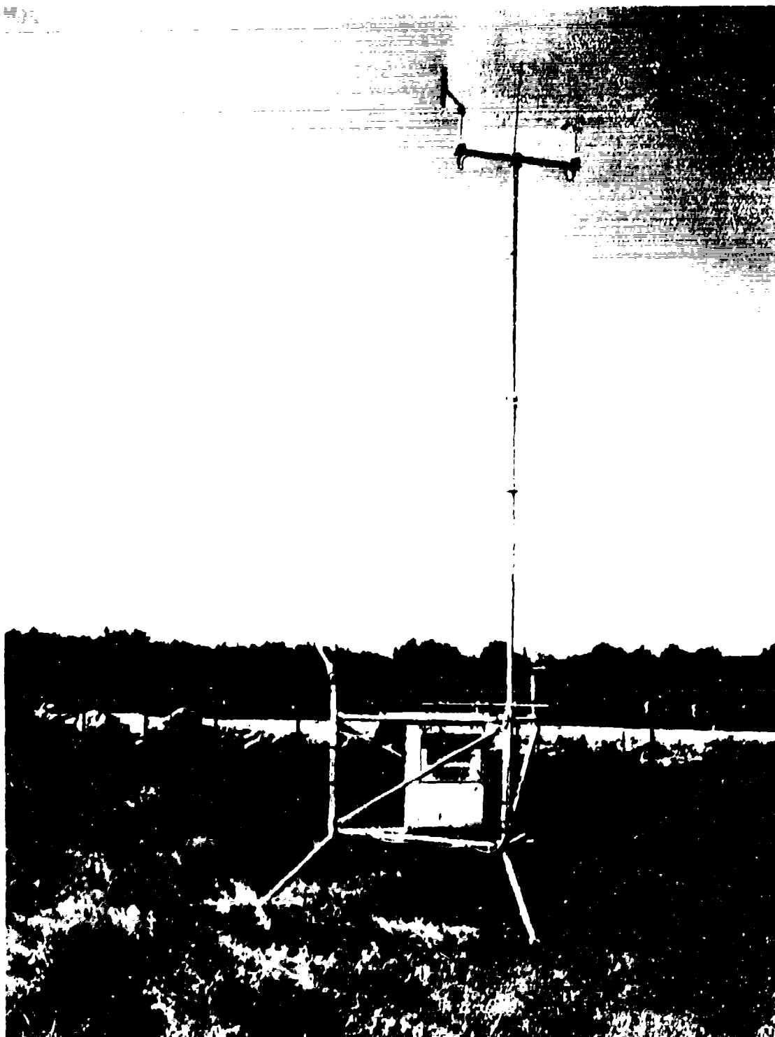
Figure 1-3 Automatic weather stations (also called mesonets) collect data on temperature, humidity, pressure, wind speed and direction 24 hours a day
