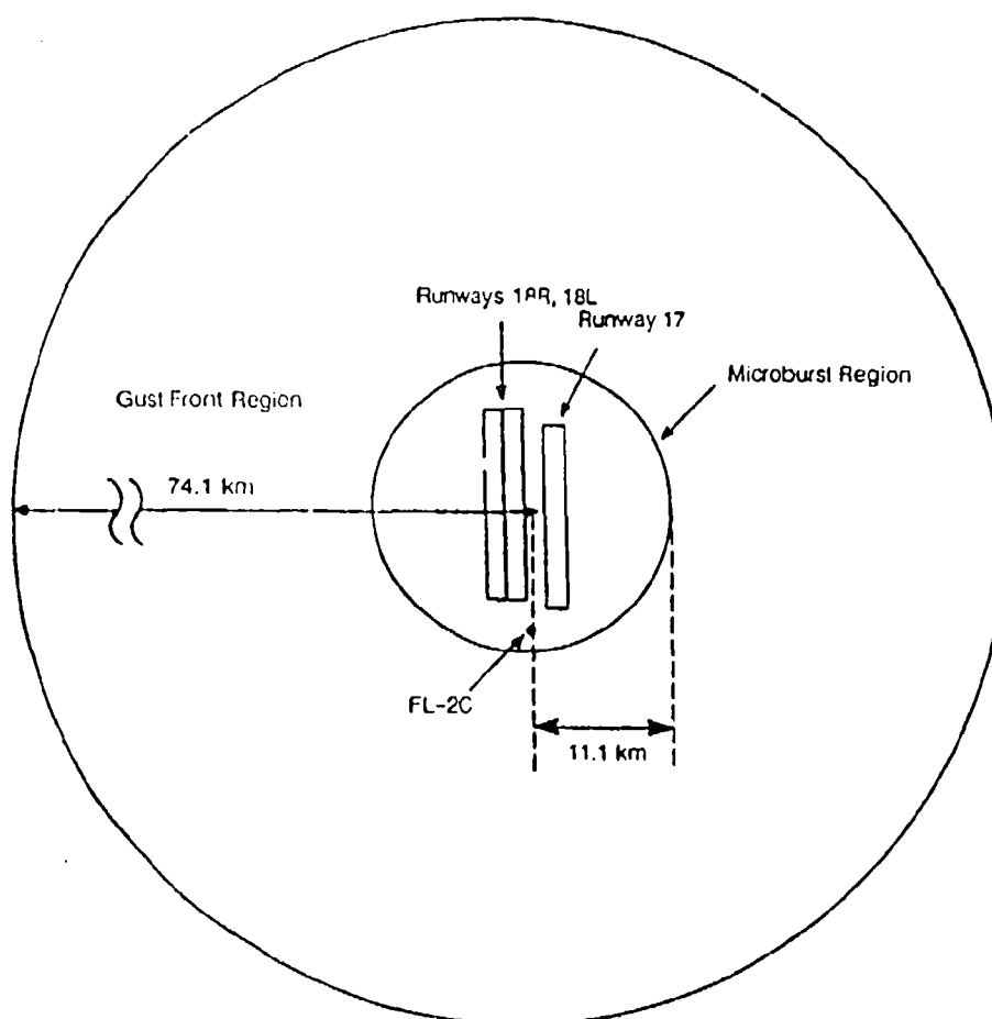
Figure 4-2. Orlando PRF selection regions.
