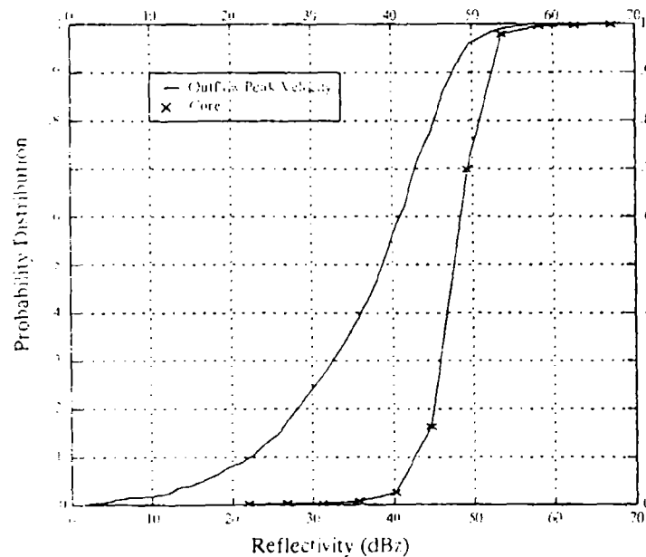
Figure 4-1. Orlando summer microburst reflectivity distribution. Solid line indicates outflow reflectivity at locations of outflow velocity maxima and minima when the microburst had its peak shear.
