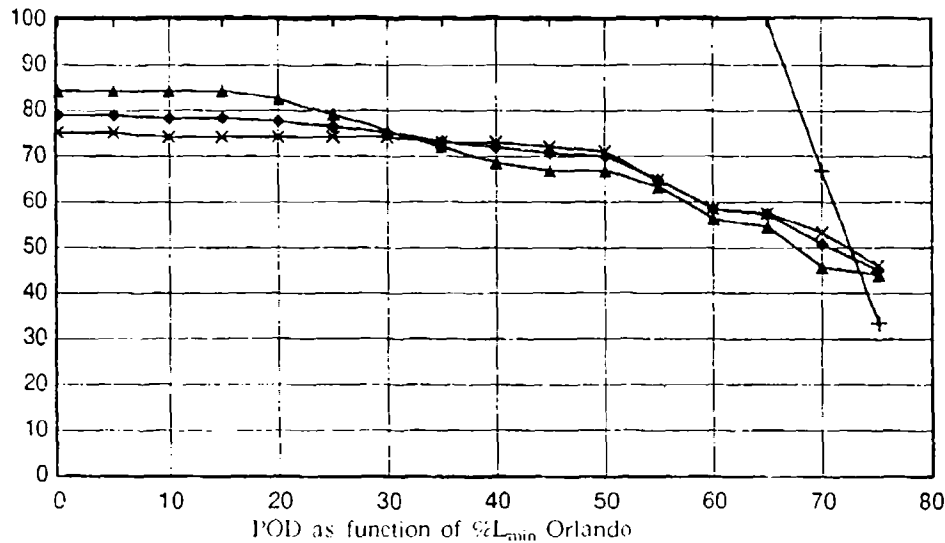
Figure 3-1. Probability of detection as a function of minimum percent of length detected threshold for moderate (x), strong (▲), severe (+) and all (◆) gust fronts.
