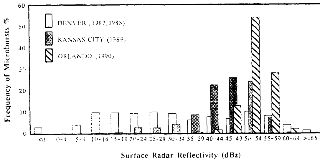
Figure 2-2. Distribution of maximum surface reflectivity in cells that produced microbursts in Denver, Kansas City, and Orlando.
