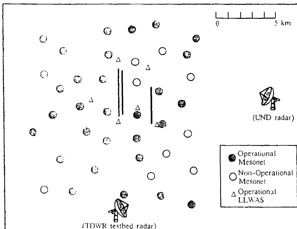
Figure A-1. Configuration and operational status of the Mesonet and LLWAS stations in Orlando, FL during September 1990. North-south lines in the middle of the network represent the runway configuration for MCO.
