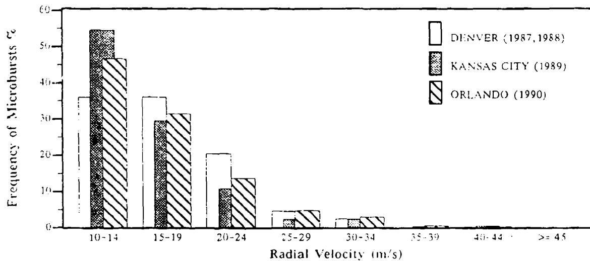
Figure 2-1. Distribution of maximum radial outflow velocity for Denver, Kansas City, and Orlando microbursts.
