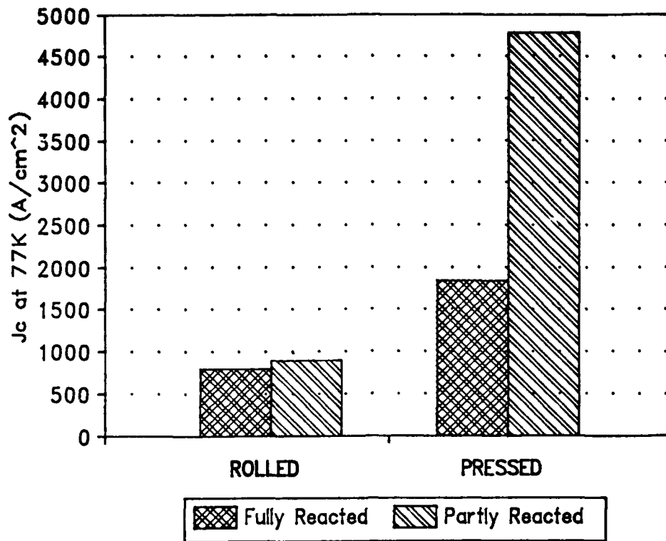
Figure 1 Critical current density of BSCCO-Ag tapes at zero applied field. Demonstrates the effect of initial powder 2223 content and final deformation method on Jc. Tapes were swaged, drawn, and rolled to 0.25mm thickness and heat treated 48hr at 830 o C in air. They were then either rolled to 0.125mm or pressed followed by a second identical heat treatment
