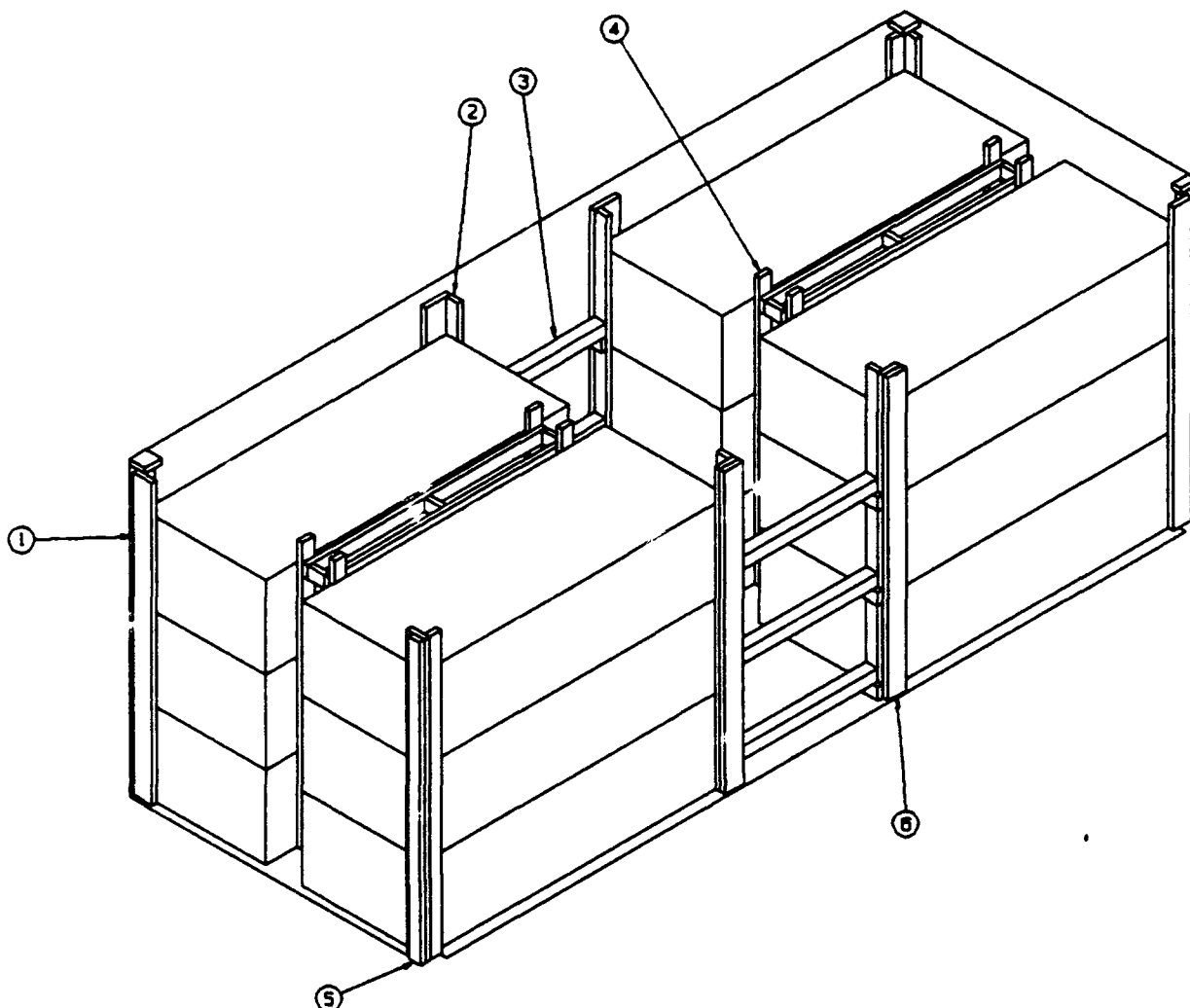
ISOMETRIC VIEW
