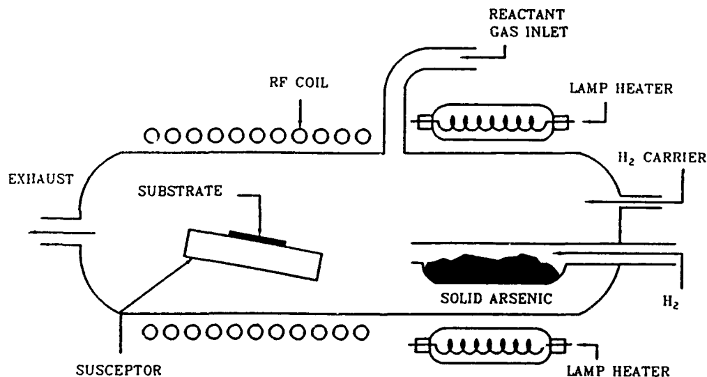
Figure 3.2 The horizontal reactor for the MOVPE growth of GaAs using elemental arsenic.
