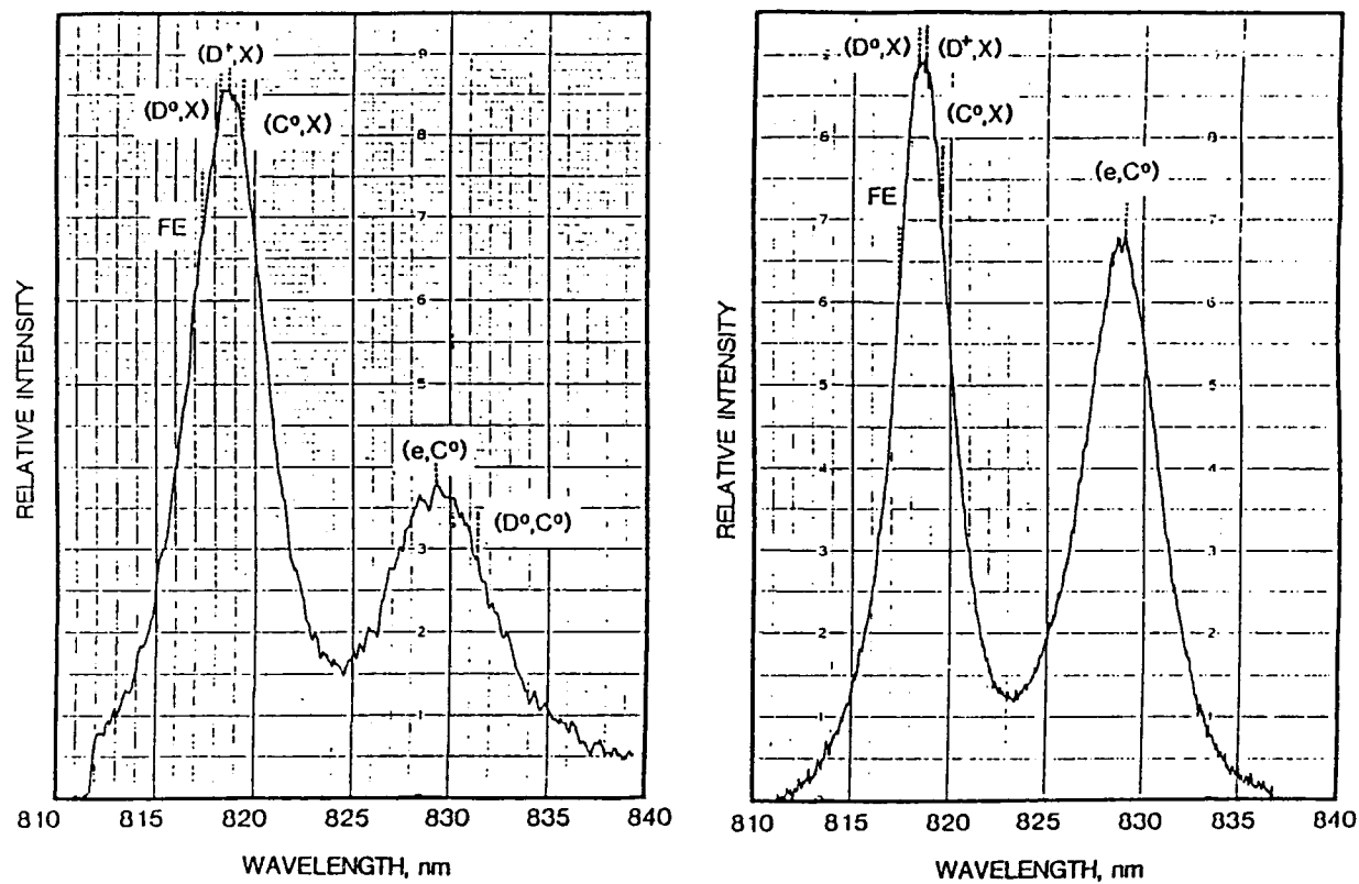
Figure 4.5 4.2 K Photoluminescence spectra of epitaxial GaAs films grown by laser-enhancement at fluences of 20.8 (left) and 23.6 (right) mJ/cm².
