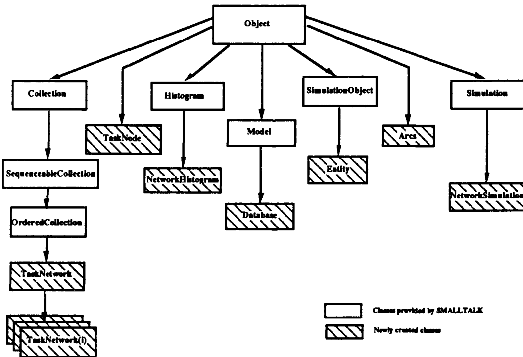
Figure 7c. Class Hierarchy of the Network Simulator
