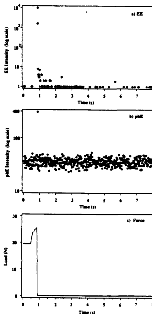
FIG. 2. (a) Electron emission, (b) photon emission, and (c) measured load accompanying the peeling of an Au film from an Si substrate with a native oxide. The sharp drop in the load curve shows the time of fracture.
