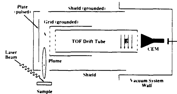
FIG. 2. Diagram of apparatus to direct a pulse of charge from the laser plume through the TOF tube.
