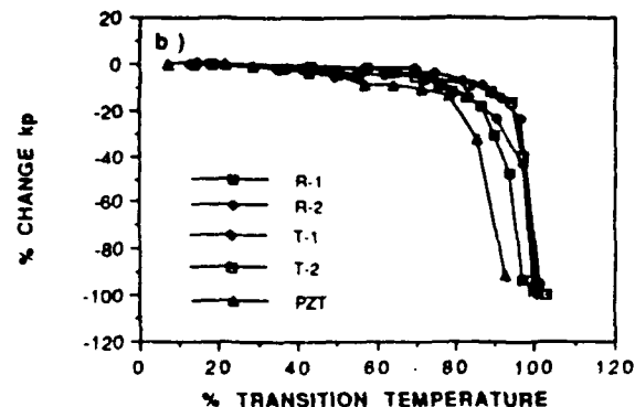
Figure 4. The % change in radial coupling factor k_p for rhombohedral compositions R-1, R-2 and tetragonal compositions T-1, T-2: a) as a function of temperature ; b) as a function of % transition temperature.
