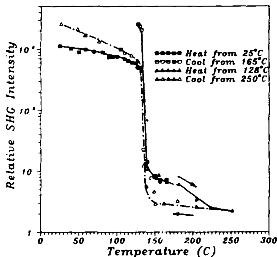
Fig. 3. Relative SHG intensity versus temperature for a multidomain single-crystal fiber of \text{BaTiO}_3 .
