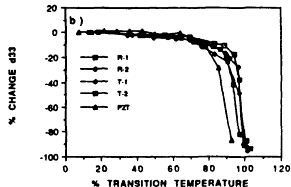
Figure 5. The % change in d_{33} piezoelectric charge coefficient for rhombohedral compositions R-1, R-2 and tetragonal compositions T-1, T-2: a) as a function of temperature ; b) as a function of % transition temperature.
