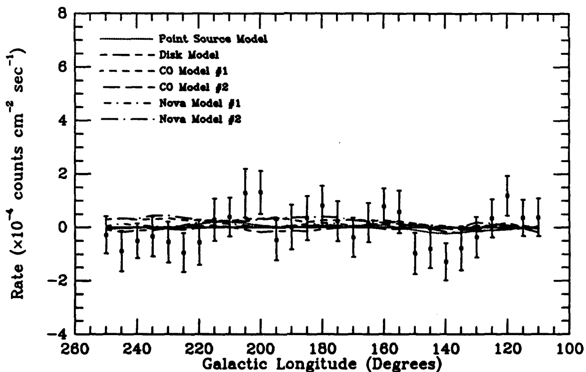
Figure 3: The background corrected counting rates for observations of positions in the direction of the Galactic Center ( upper ) and the Galactic Anti-center ( lower ). Note that this does not represent the distribution of the 1.809 MeV radiation. Also shown are the expected responses for each of the ^{26}\text{Al} distribution models.
