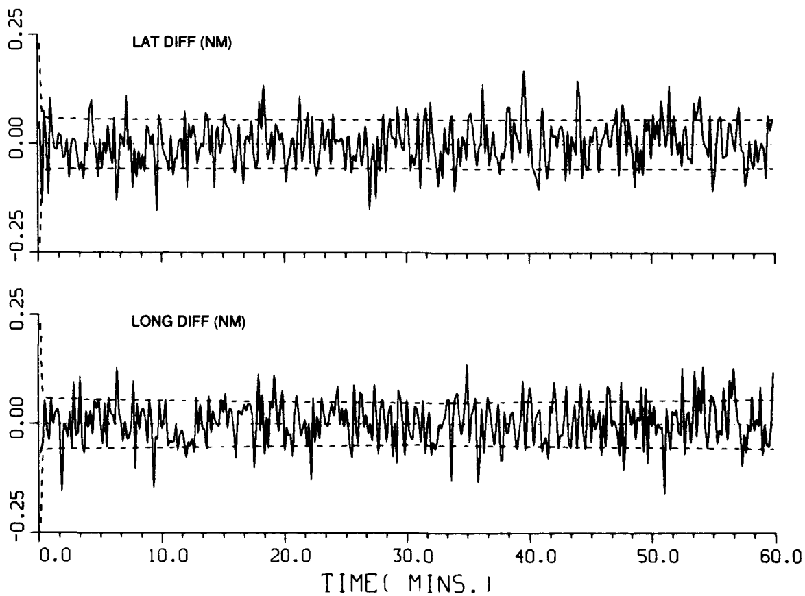
FIG. 24: INNOVATIONS FOR KALMAN FILTER POSITION MEASUREMENTS
