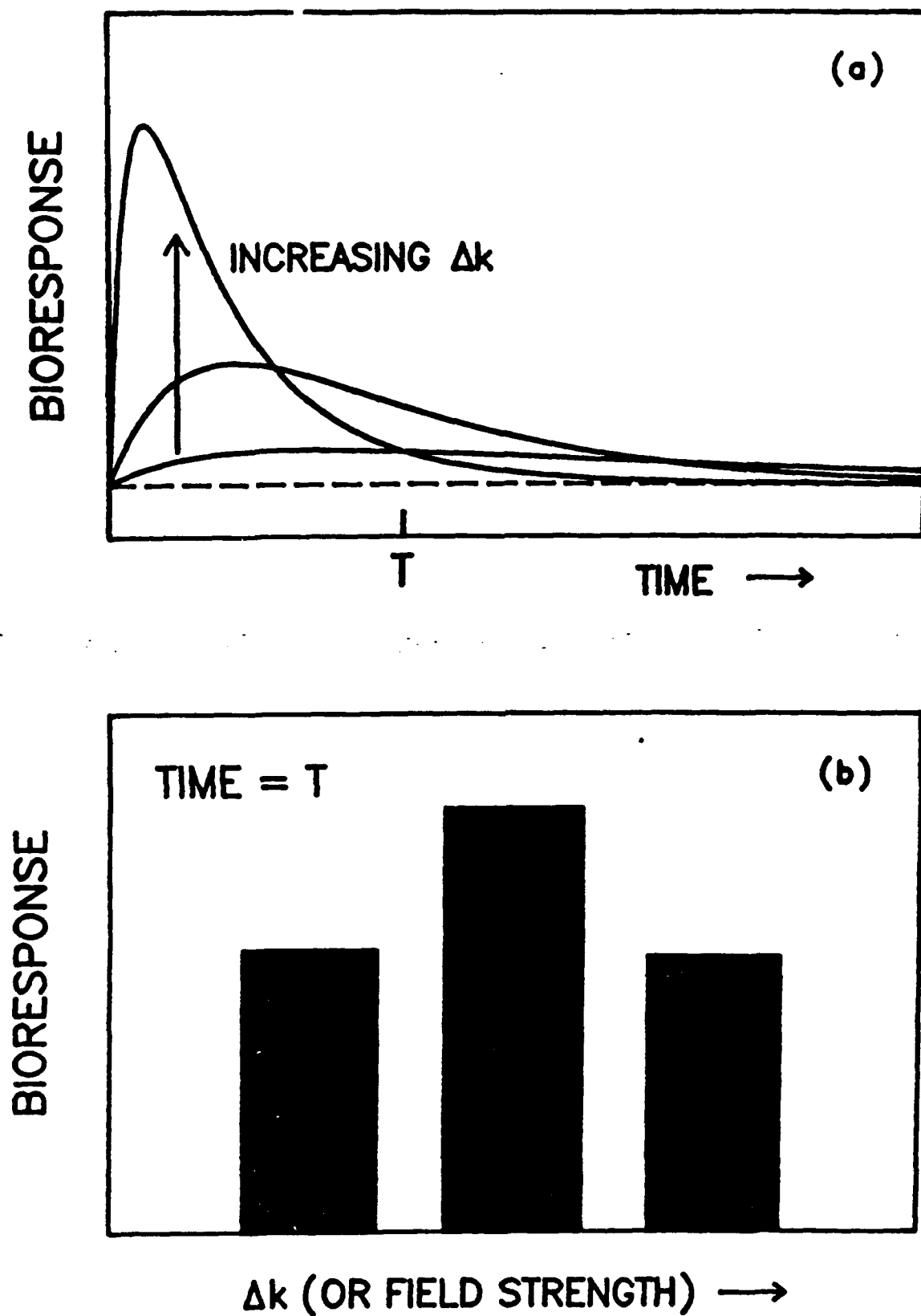
Fig. 1.2. (a) The prediction of the multi-step model for the time evolution of the concentration y(t) following the switching on of the exogenous electromagnetic field at time = 0. The curves are calculated from equation (1.4) for three values of \Delta k . (b) The apparent "power window" that results when measurements are made as a function of field strength (here characterized by increasing \Delta k ) at one specific time, T in (a), after exposure is initiated.
