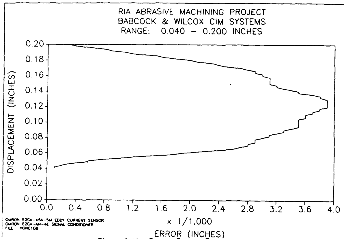
Figure 3-19, Omron Sensor Errors
