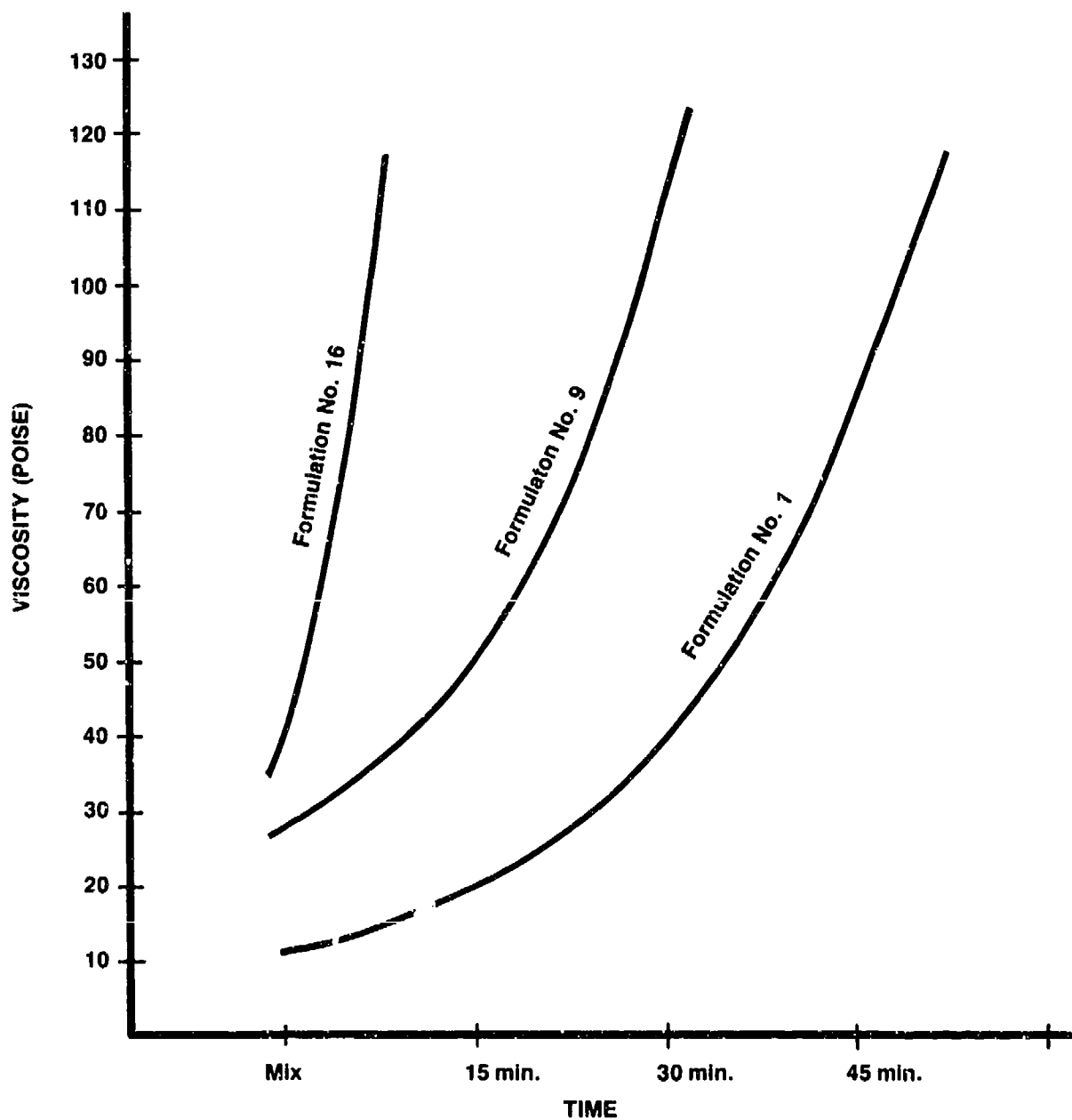
FIGURE IV Rate of Cure Expressed by Viscosity Change At 15 Minute Intervals at 140°F (60°C)
