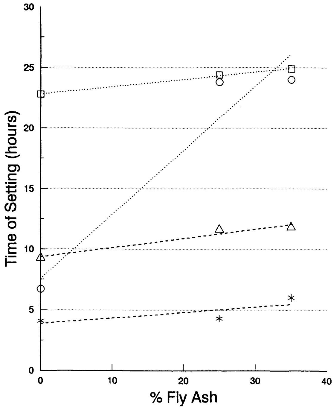
temp=50 temp=80 temp=50 temp=80 no CaCl 2 no CaCl 2 2% CaCl 2 2% CaCl 2 .....□..... ---△--- .....○..... ---*--- Figure 2. Final time of setting versus percent fly ash at 50° and 80° F, with and without CaCl 2
