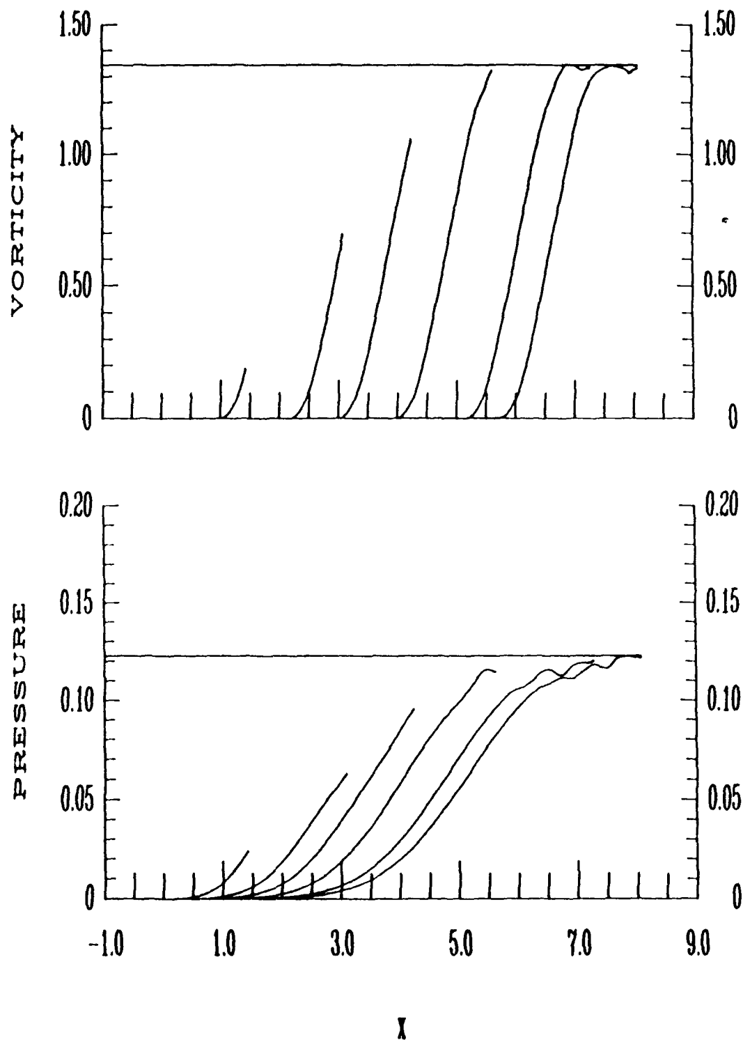
Figure 3d. Response to a 10% disturbance with slow ramping. R = 6 , \alpha = 2 , and \theta = 40^\circ . The curves correspond to t = .237, .512, .704, .933, 1.208, 1.342 .
