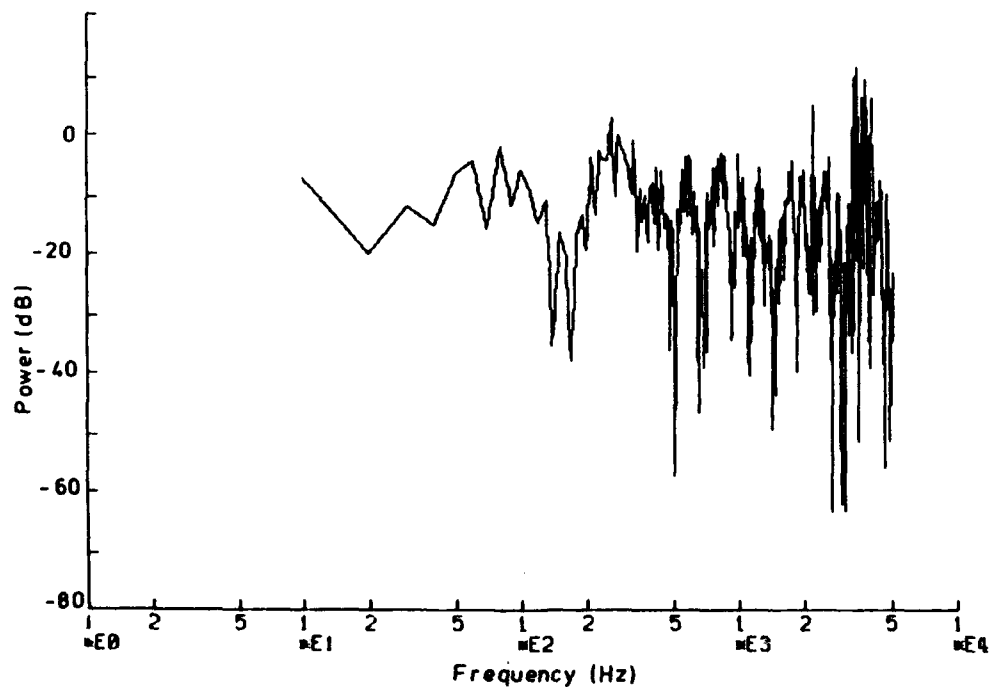
FIGURE 13 POWER SPECTRUM OF TOTAL PRESSURE (0-1024)
