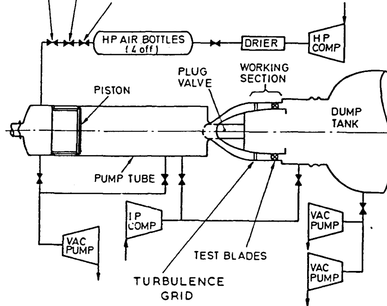
FIGURE 1 THE ILPC TEST FACILITY
