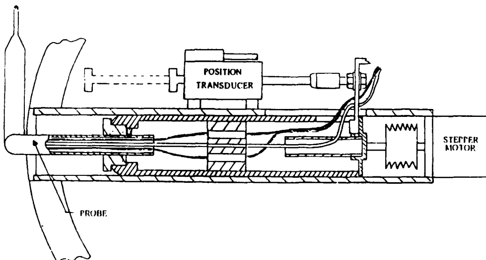
FIGURE 11 PROBE RADIAL DRIVE
