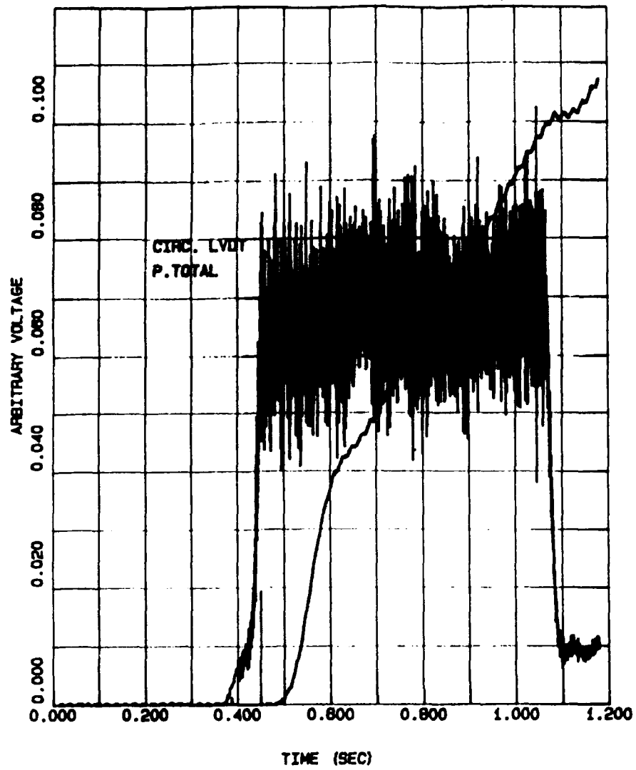
FIGURE 12 UNFILTERED TOTAL PRESSURE
