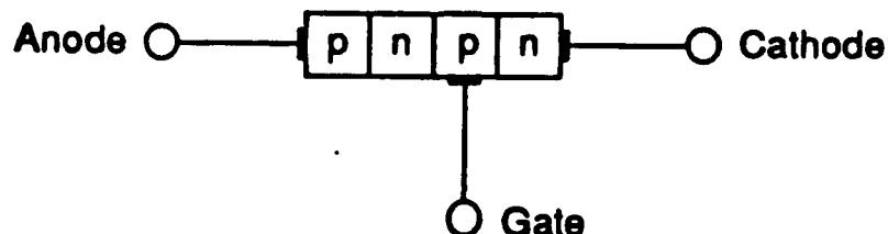
Figure 16. SCR Construction
