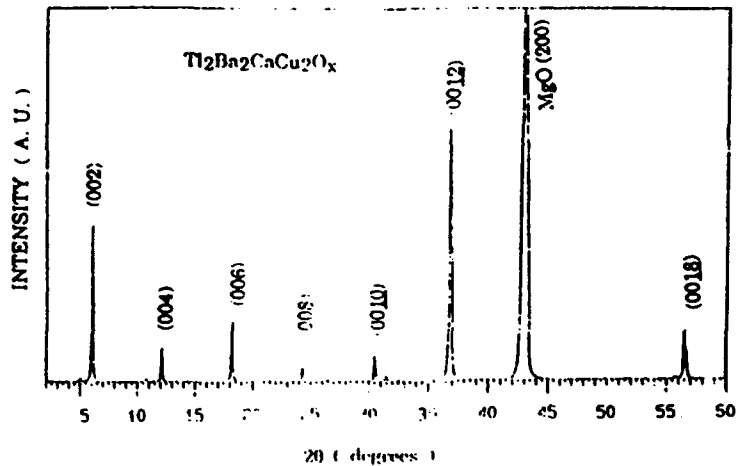
Figure 5. X-ray diffraction curve. The film is highly c-axis oriented Tl_2Ba_2CaCu_2O_x .
