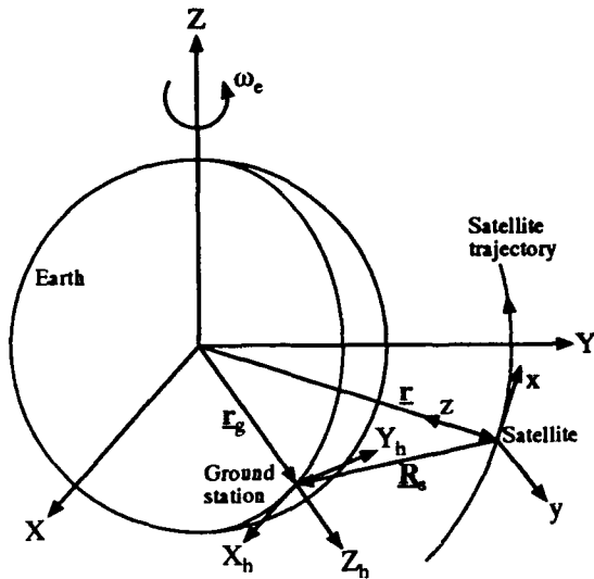
Fig 1(a) — The geocentric, topocentric, and vehicle-centered coordinate frames. \underline{\omega} = \omega_e \mathbf{K} is the angular velocity of the rotating Earth. This figure is not drawn to scale.
