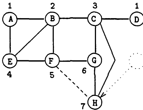
Figure 3: Example Network with Mobile Node
