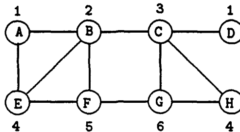
Figure 2: Example Network Using Node Allocation
