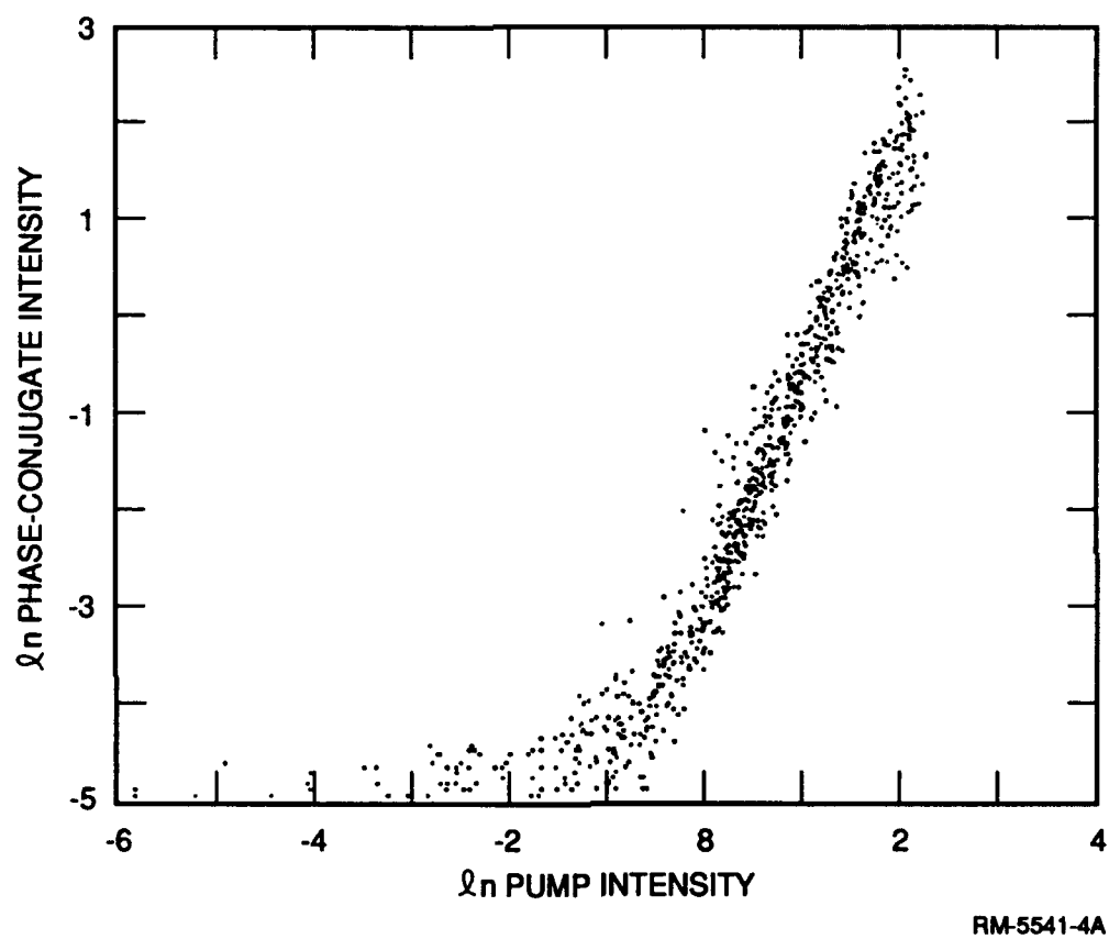
Figure 7. Typical phase-conjugate signal as a function of laser intensity (6350 Å, 2-ps pulse length.)
