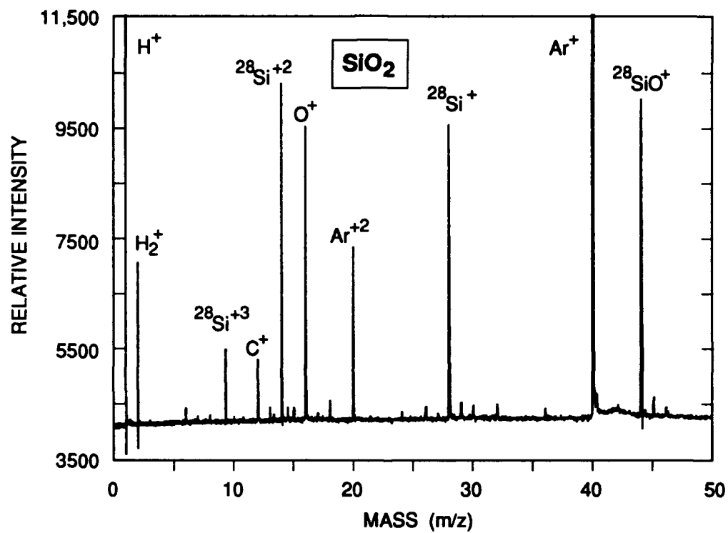
Figure 8. Time-of-flight mass spectrum from photoionization of neutral component released from SiO_2 substrate following ion bombardment. ( 6400\text{\AA} , 500 fs, 1 \times 10^{14} \text{ W/cm}^2 ).
