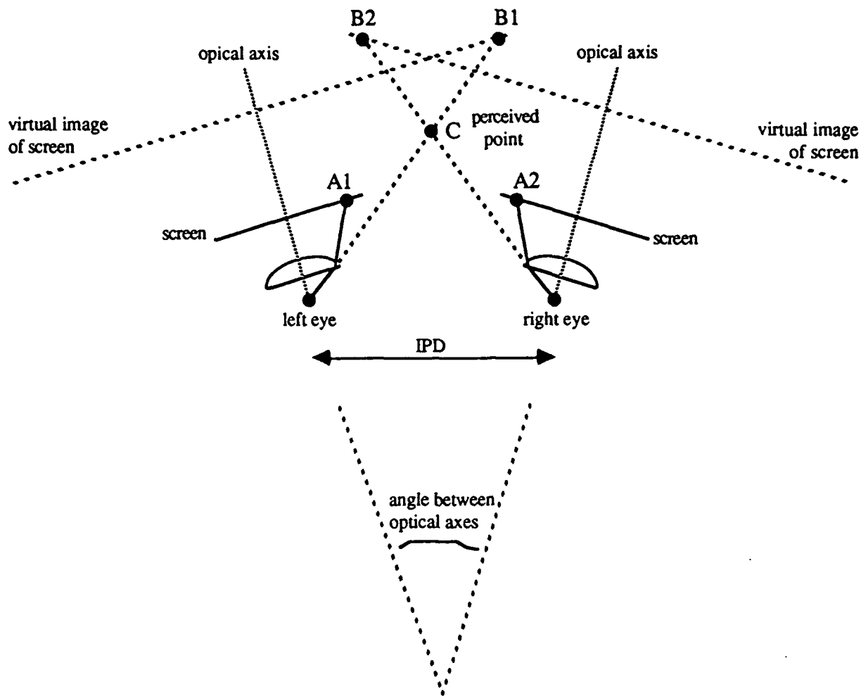
Figure 3.2 Stereoscopic optics model
