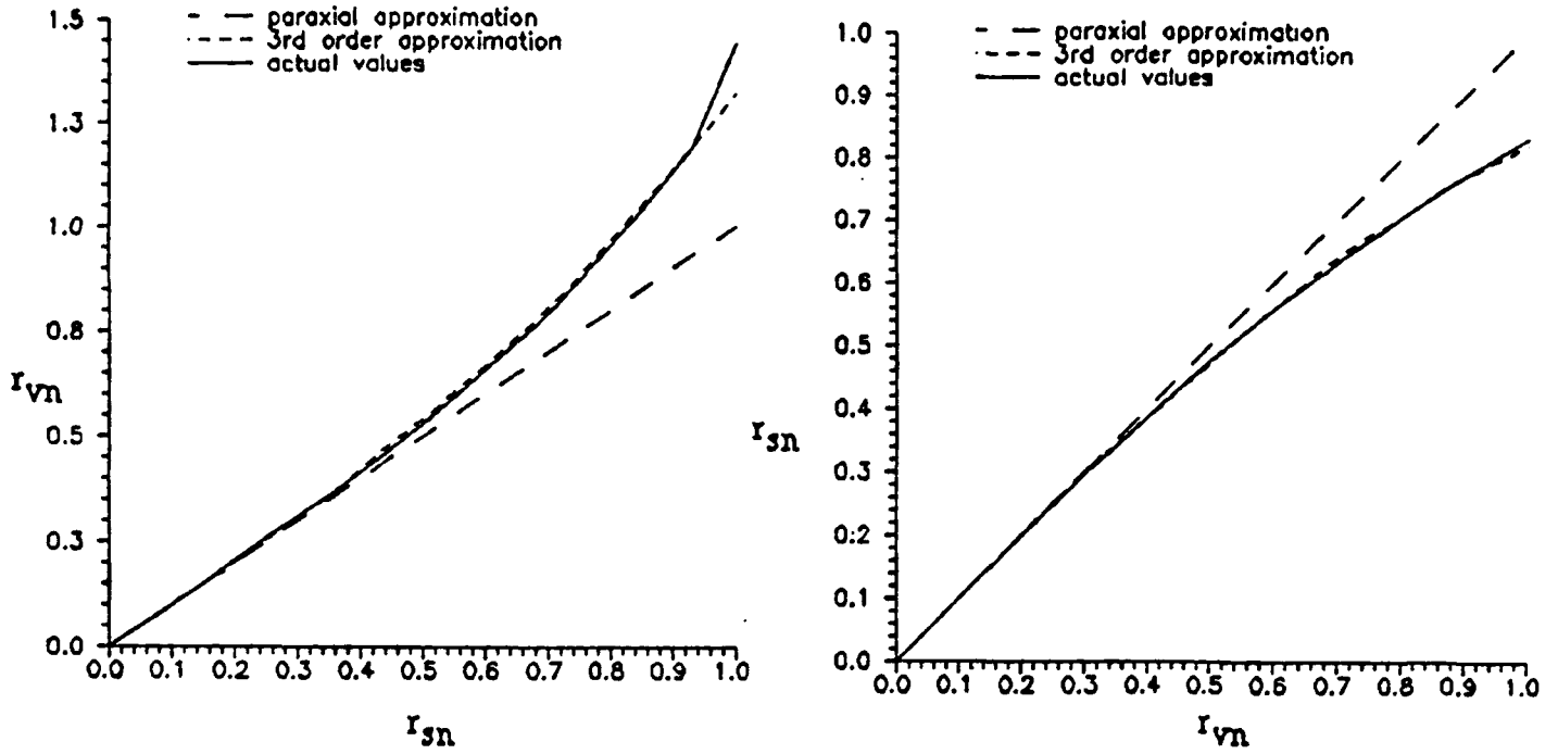
Figure 4.4 Graph of r_{vn} vs. r_{sn} for D ( k_{vs} = 0.32 ) and ray-tracing for the LEEP optics; graph of r_{sn} vs. r_{vn} for D^{-1} ( k_{sv} = -0.18 ) and ray-tracing
