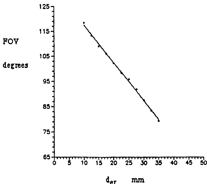
Figure 4.6 Graph of FOV vs. d_{er}
