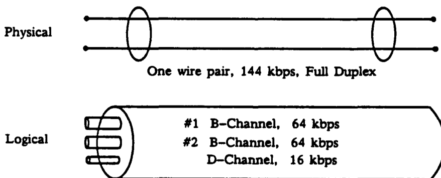
Fig. 5 ISDN Basic Rate Access
