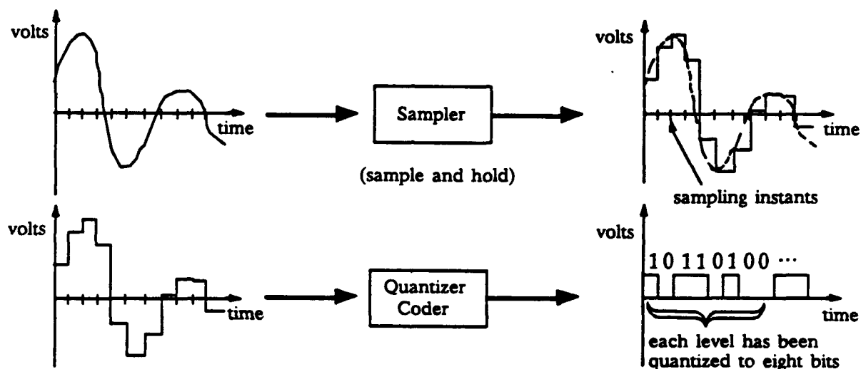
Fig. 2 Analog-to-Digital Conversion
