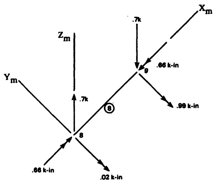
Internal Forces of Typical member ⑧ Member Axes
