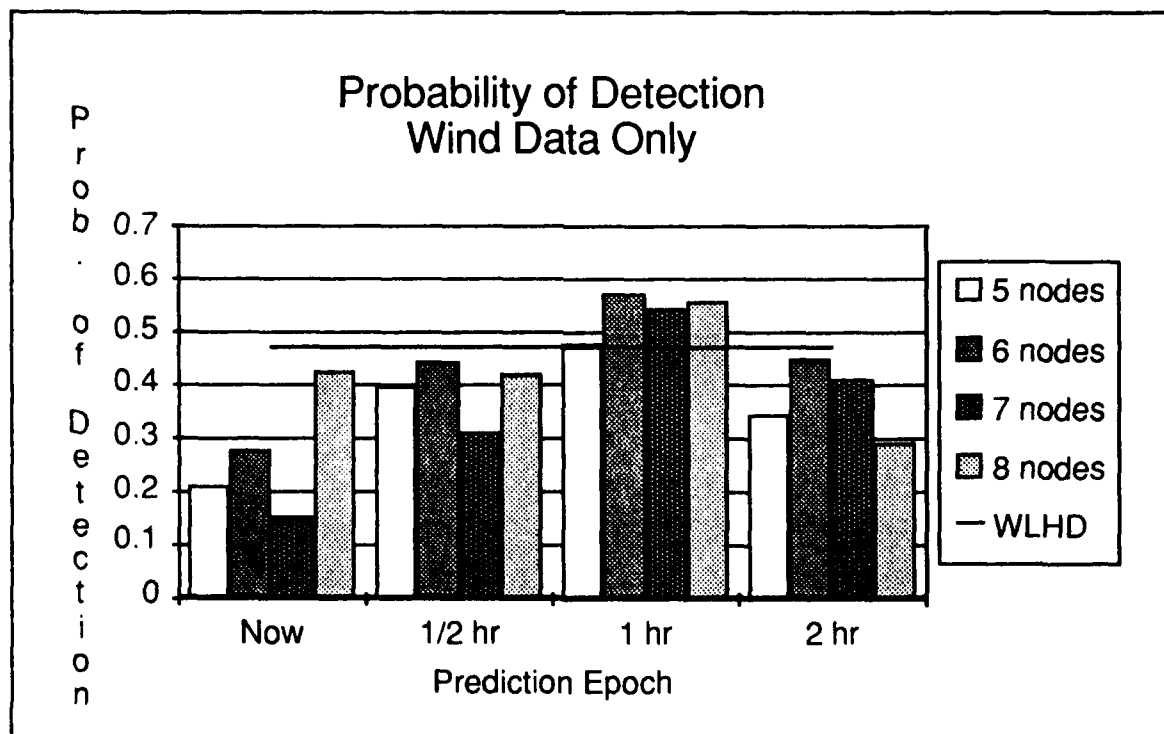
Figure 4-1 Probability of detection by time epoch of the ANS using two days of wind data as input. The horizontal line labeled WLHD is the level of performance of Watson et al. 1987 in predicting lightning for the entire KSC area at any time following a threshold crossing of the Total Area Divergence.
