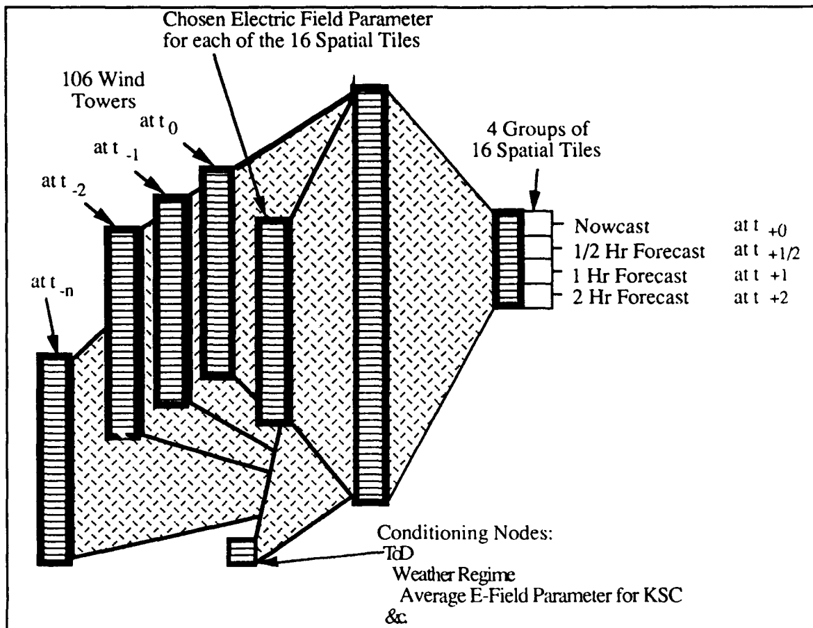
Figure 3-1 Electric Field added to the spatial array (16 nodes) and the 'conditioning' nodes (1 node) inputs for a \{p + 16 + [106 \times n]\} \times m \times 64 backpropagation network proposed for using electric/wind tower histories in forecasting KSC lightning strikes.
