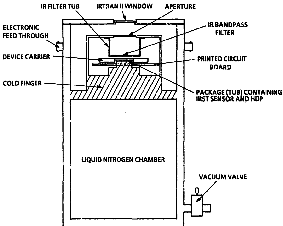
Figure 6-2. Cross section of 9-inch-diameter CIM LN 2 Dewar assembly, shown in assembly position (upside down).
