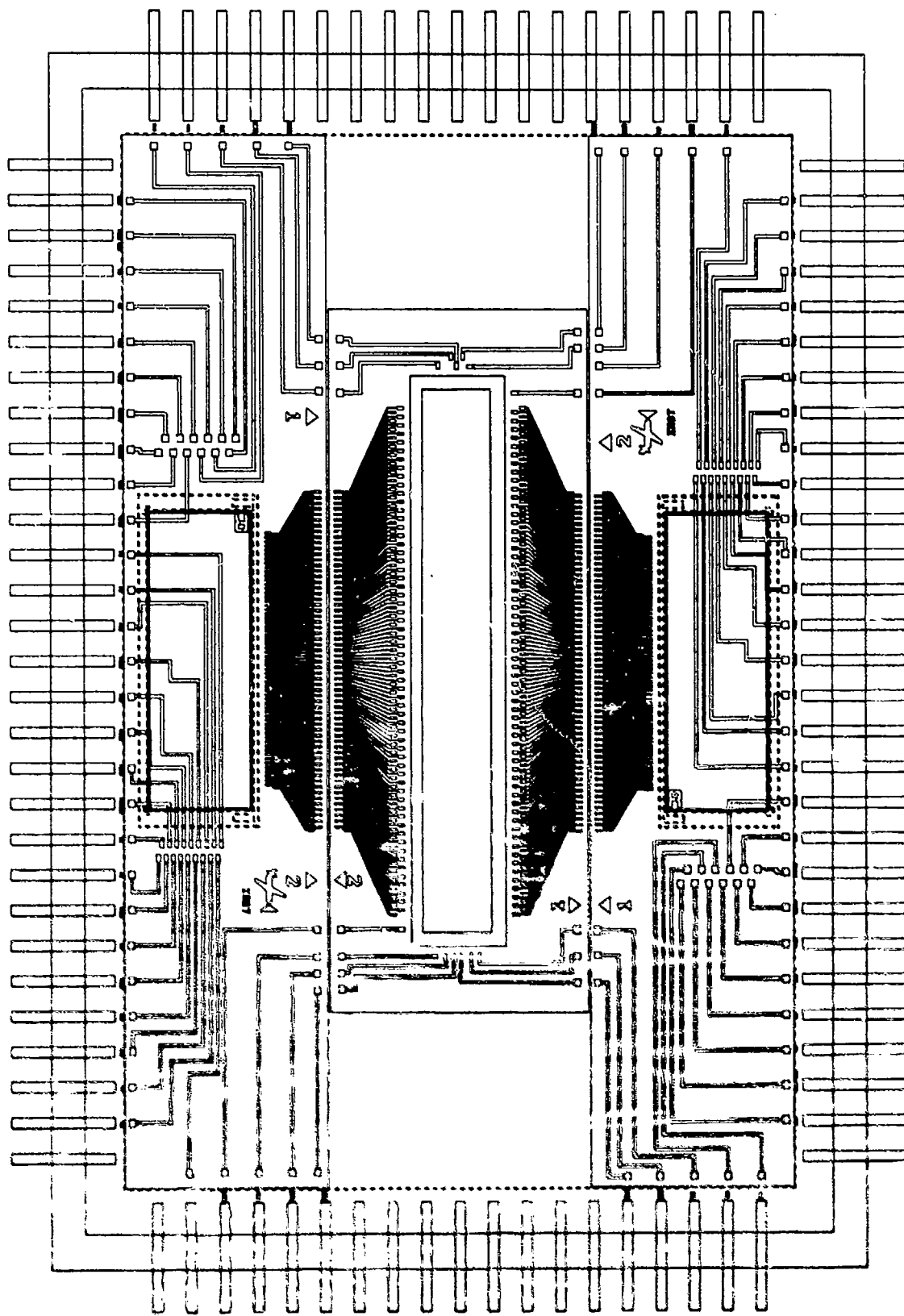
Figure 6-9. IRST composite carrier design in standard 96-pin package layout.
