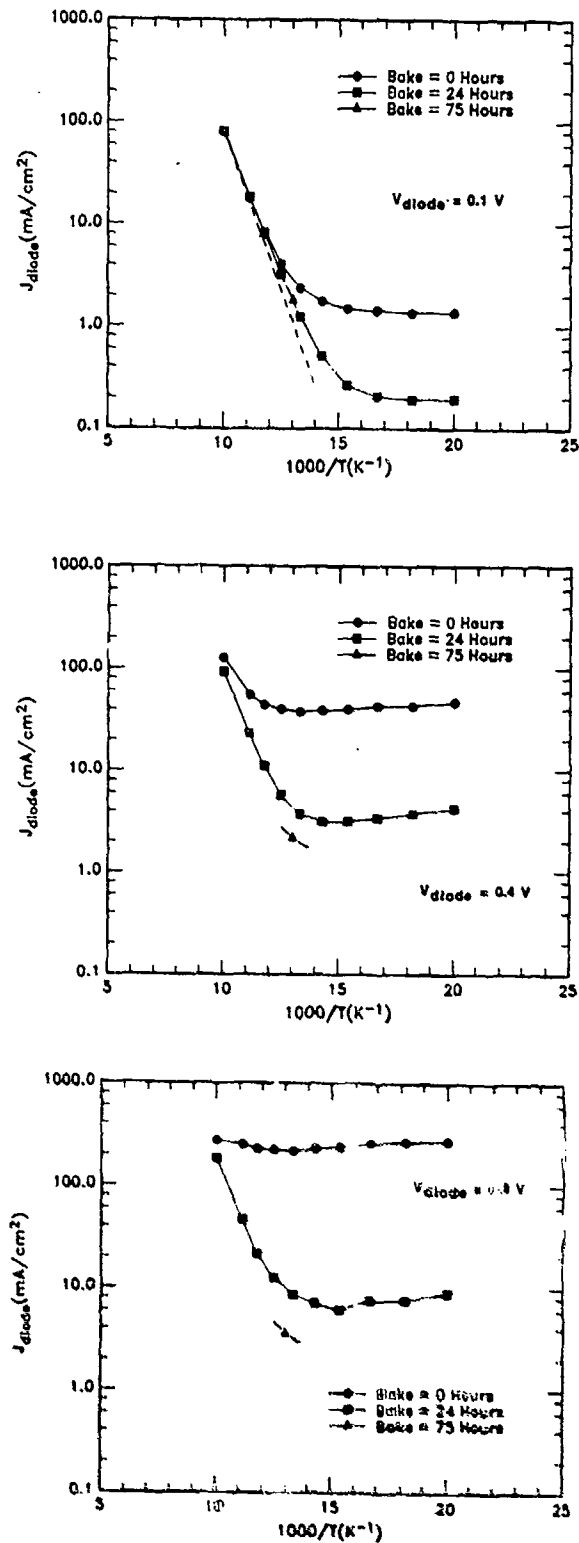
Figure 3-10. Leakage current density for diode 26-2-1U-LPB as function of inverse temperature at three stages of postannealing for three reverse-bias levels. Measurements following final bake (75 hours) were made at 77 K only. Dashed line in upper figure is for diffusion-dominated leakage mechanism.
