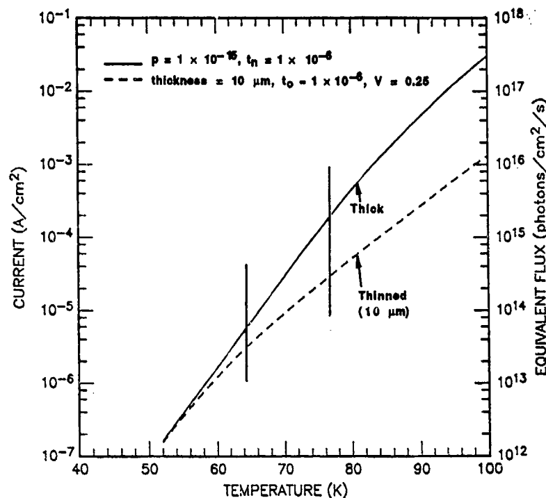
Figure 3-17. Model calculation of MIS dark-current density versus temperature for unthinned (bulk) and thinned (10- \mu\text{m} thickness) p-type HgCdTe of 10 \mu\text{m} cutoff. Vertical markers are at 65 K and 77 K. The calculation for thinned substrate assumes an accumulated back surface.
