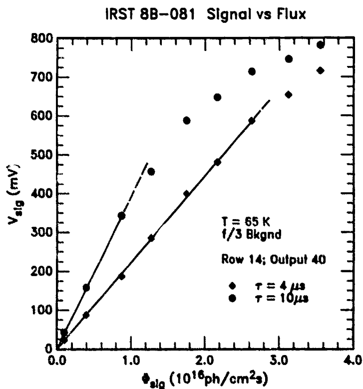
Figure 7-13. Responsivity data for same detector element of Figure 7-12 for two different integration times. ( T = 65 K).
