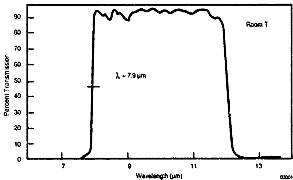
Figure 6-15. IR transmission spectrum of IRST cold-shield bandpass filter assembly.
