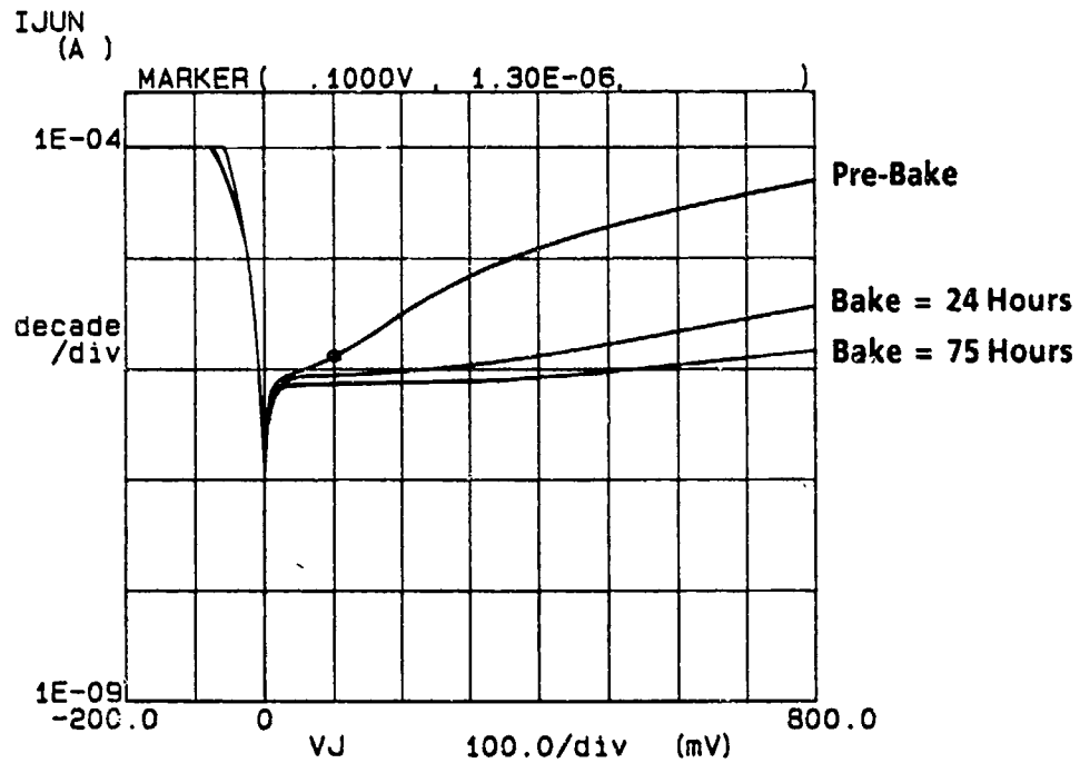
Diode 26-2-CU-LPA
