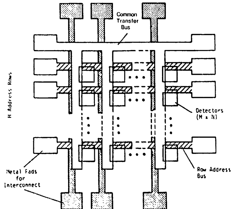
Figure 2-3. Schematic CIM detector array.
