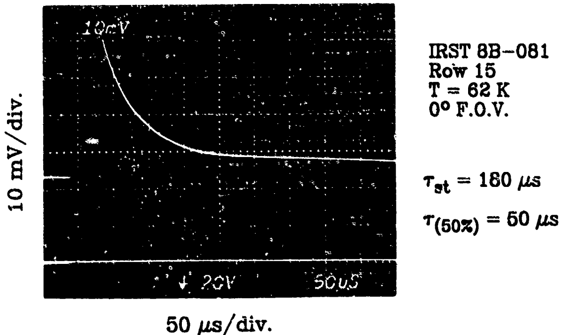
Figure 7-5. MIS charge-storage characteristic for one row of IRST 8B-081 at T = 62\text{ K} and 0\text{-degree FOV} .
