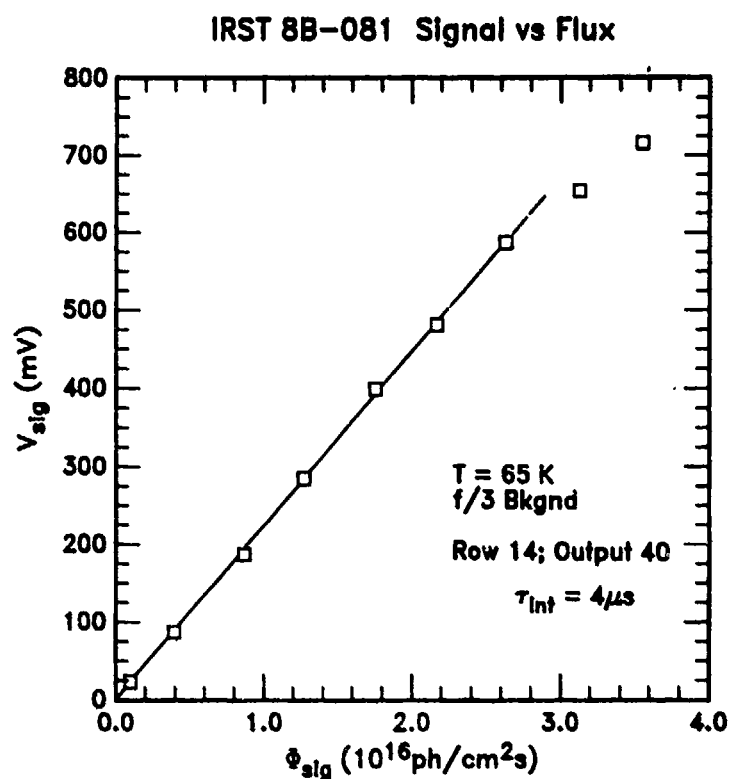
Figure 7-12. Response versus 900 K signal flux for typical detector element of IRST 8B-081 at T = 65 K and f/3 FOV. Integration time was 4 \mu s . Corresponding single-pixel responsivity is 63 MV/W (output referred).
