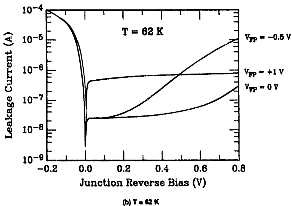
Figure 7-8. Effect of field-plate bias V_{\text{FP}} on current-voltage characteristics of a diode test structure from IRST 8B-080.
