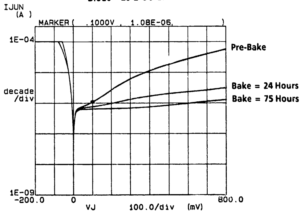
Diode 26-2-CU-LPB
