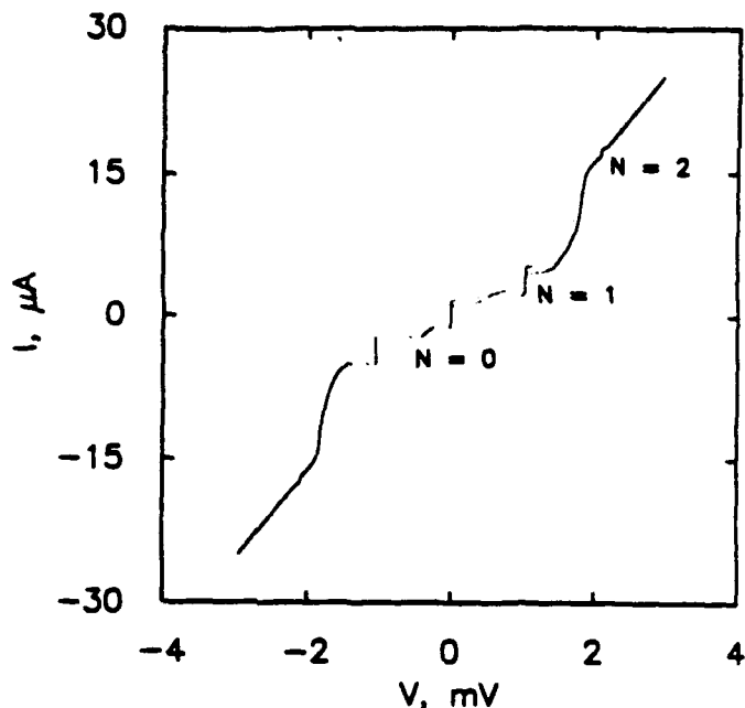
Figure 5: IV characteristic of detector junction with generator biased at V_{bias} = 1.090 \text{ mV} . The N = 1 and N = 2 Josephson steps are marked, as is the supercurrent ( N = 0 ).
