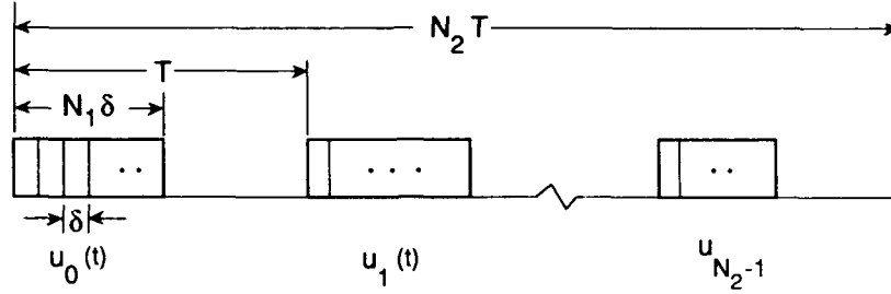
Fig. 11 — A synthesized pulse train
