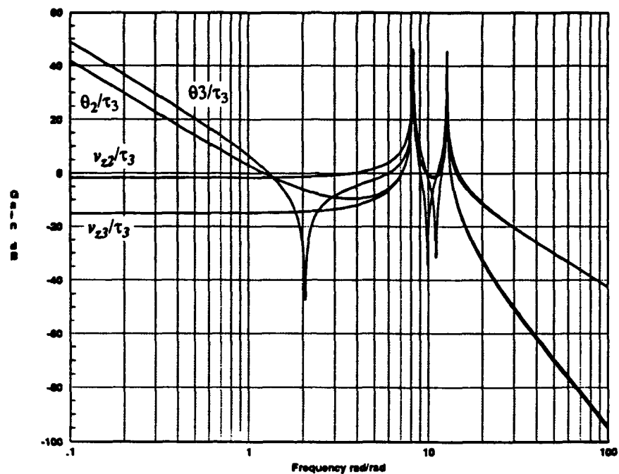
Figure 7. Body Plot of Radial Motion, \theta_2/\tau_3 , \theta_3/\tau_3 , v_{22}/\tau_3 , v_{23}/\tau_3 ( \theta_2 \sim 60 [deg], \theta_3 \sim 60 [deg])
