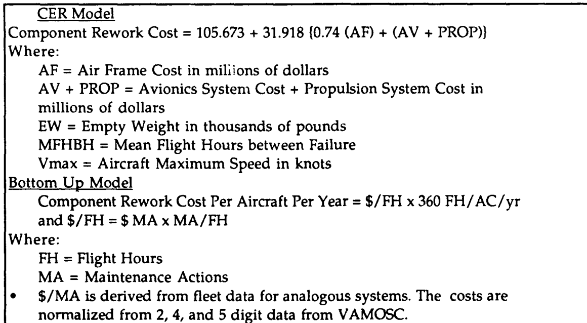
Figure 14. F/A 18 Component Rework Cost Factors Derivation [Ref. 54:p. 33]
