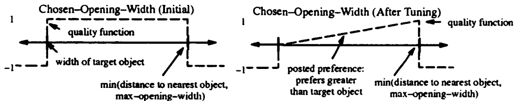
Figure 10. The Chosen-Opening-Width Parameter Quality Function After Learning New Preference
